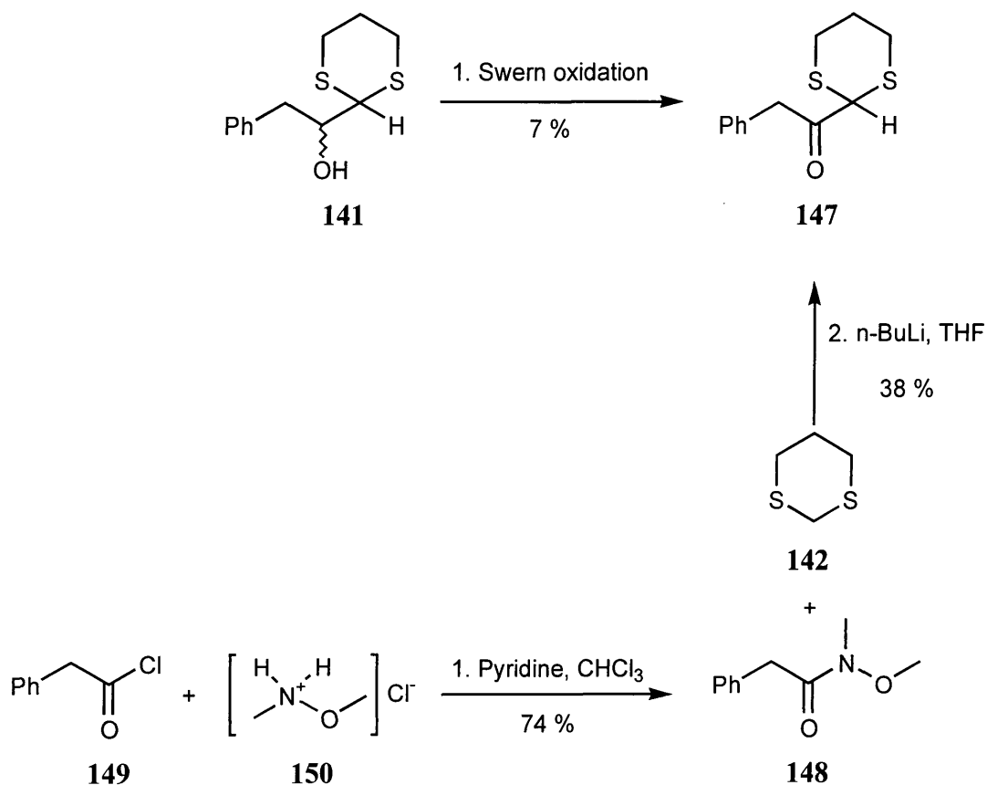
Scheme 61
