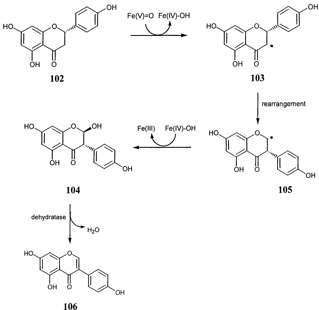
Scheme 37
