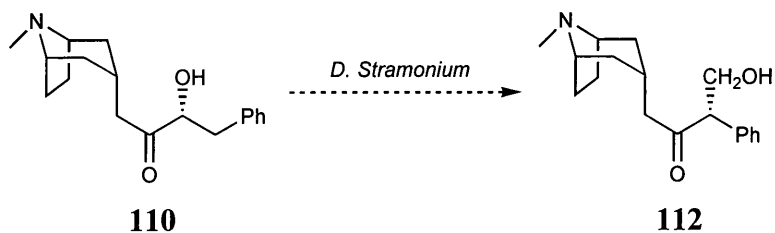
Scheme 40
