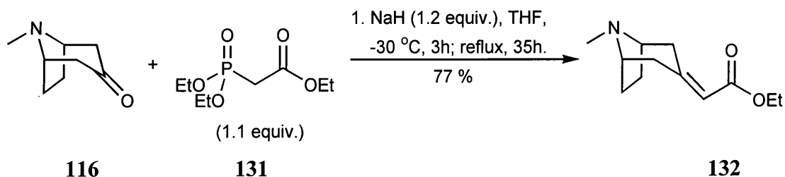
Scheme 100
