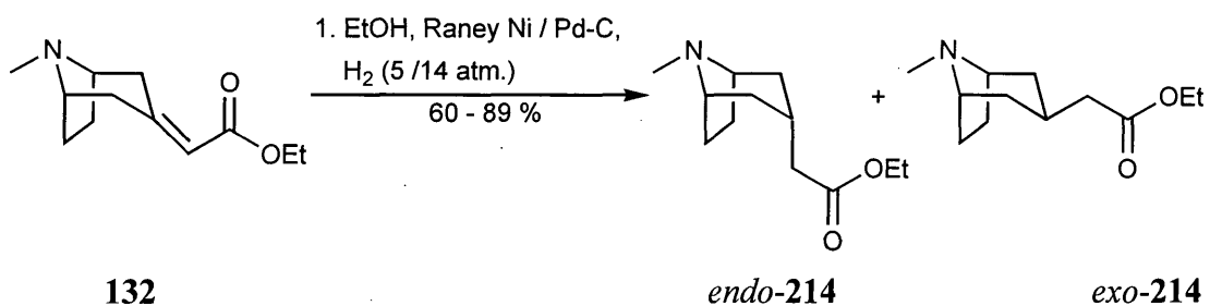
Scheme 98
