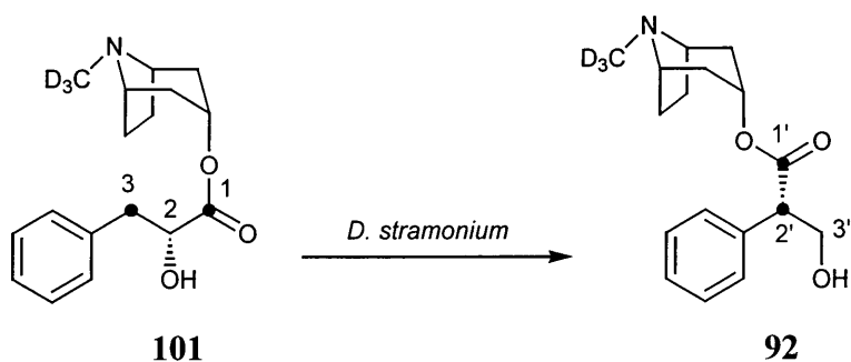
Scheme 36
