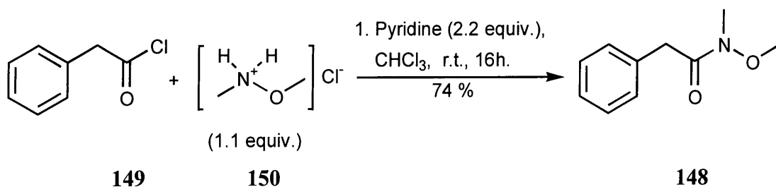
Scheme 56
