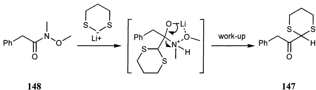
Scheme 64
