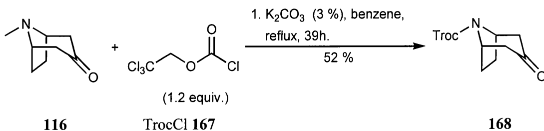
Scheme 72
