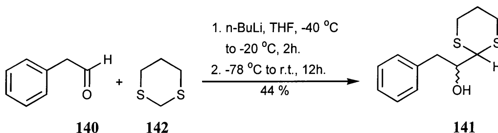
Scheme 51
