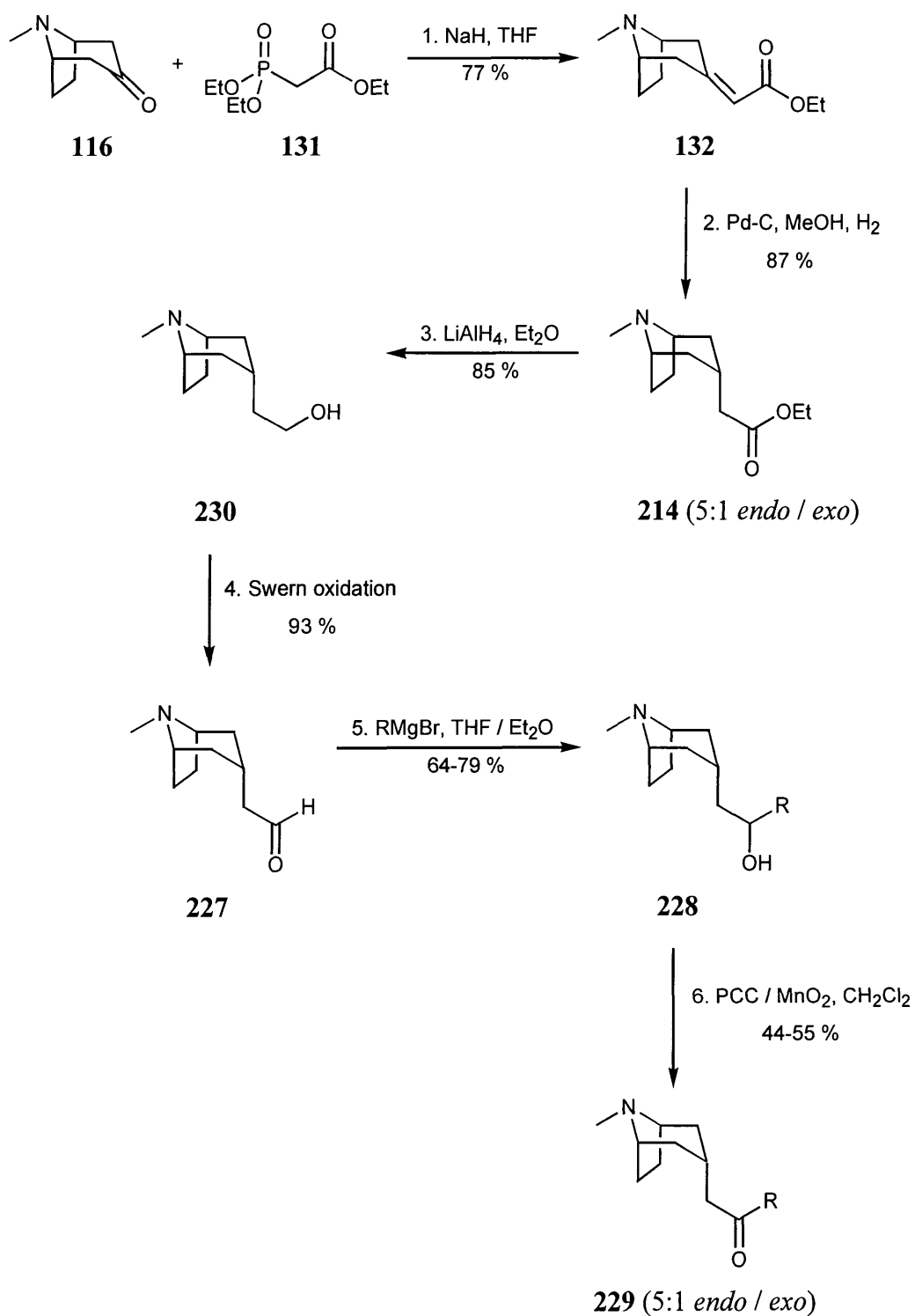
Scheme 119
