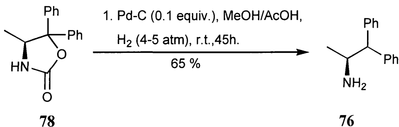
Scheme 19
