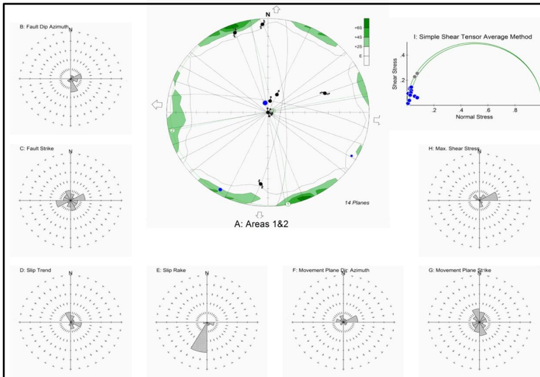
Fig. 7.12 Results of different stress phases for northwest Libya (along Al Azizyah fault zone (AZFZ), site 1&2, Jifarah Basin). Field data diagram are Schmidt's projections of lower hemisphere. A: areas 1&2. Faults are great circles, slickenside lineations are dots with arrows indicating the sense of motion of the hanging wall. Computed stress axes are represented as large blue dot ( \sigma_1 ), medium blue dot ( \sigma_2 ) and small blue dot ( \sigma_3 ). Large divergent white arrows indicate the horizontal extensional stress direction ( \sigma_3 ) whilst large convergent black arrows indicate maximum principal stress axis ( \sigma_1 ). Rose diagrams for the structures observed northwest Libya (Jifarah Basin and Nafusah Uplift). The radius of the rose corresponds to the class with the highest frequency as represented in the figure (B to I).
