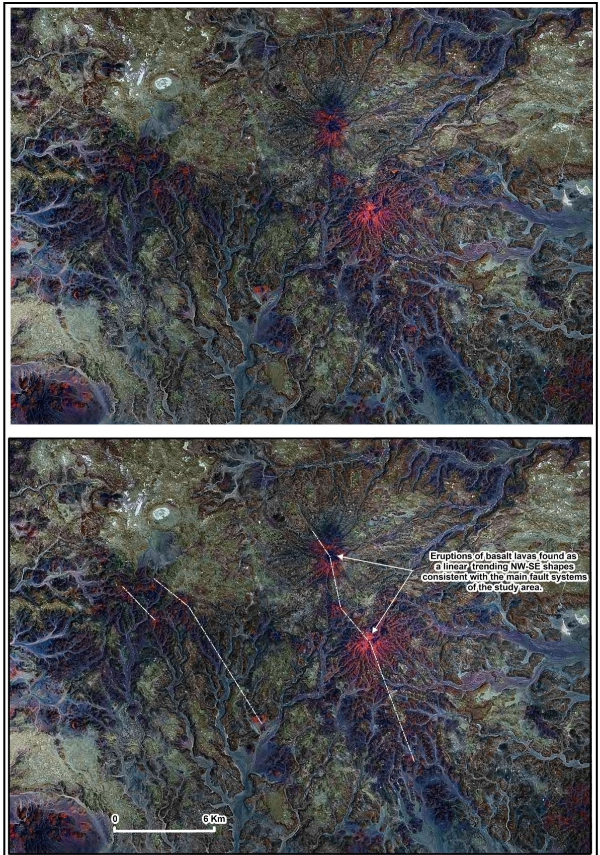
Fig. 4.8 Example of basalt lavas eruptions which found in the southern part of the study area form linear trending NW-SE shapes consistent with the main fault systems of the study area. For location see fig. 4.5.
