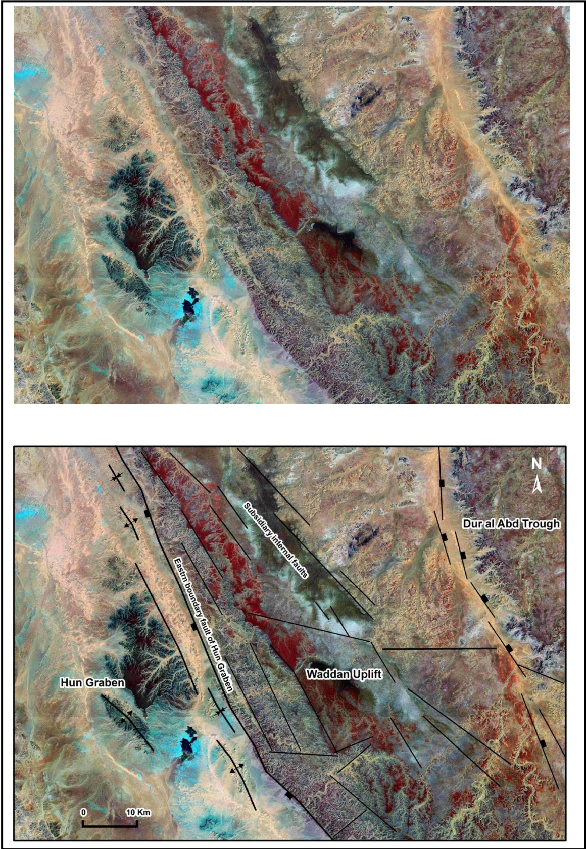
Fig. 4.24 Satellite (MrSid) imagery showing the shape of wadis (valleys) reflect the deflection of the drainage channels along the bedding contact between relatively hard and soft lithological units, at the central part of Waddan Uplift (For location see Fig. 4.5).
