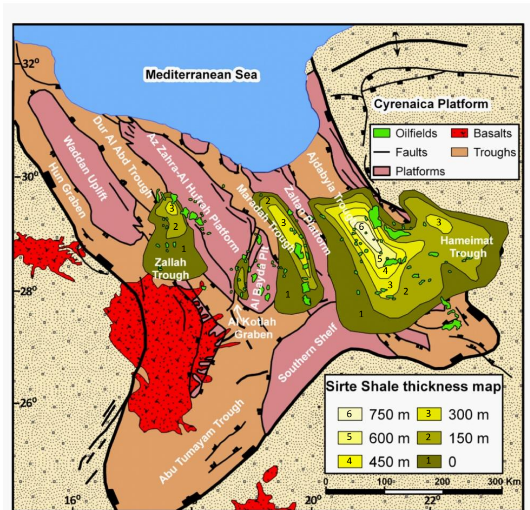
Fig. 3.1 Sirte Shale thickness map of Sirt Basin. Modified after El Alami et al, (1989); Rusk, (2001); Ahlbrandt, (2001); Hallett, (2002).
