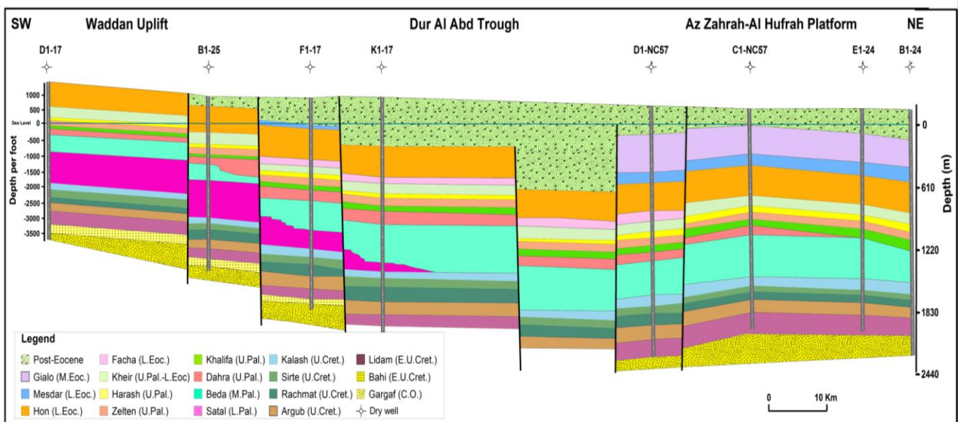
Fig. 6.7 Geological cross section A-A' view of present day structure across the study area from the southwest to the northeast (See figure 1.4 for location).
