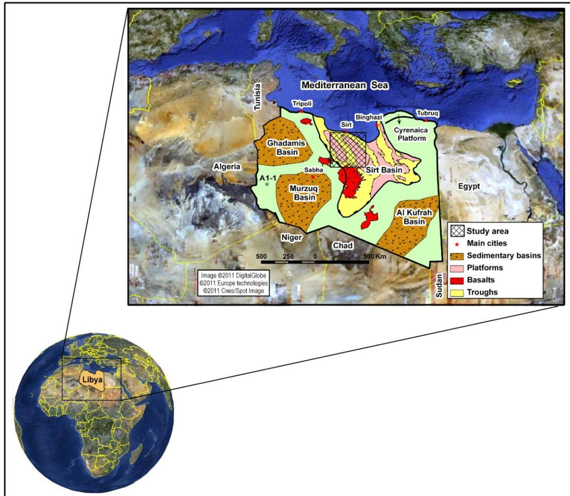
Fig. 1.1 Generalized tectonic map of Libya as located in the north central Africa showing the major structural elements and main sedimentary basins of Libya (modified after Mouzugi, and Taleb1981 and Abadi, 2002). Marked box represents the study area. Well A1-1 is shown in the northwestern Murzuq Basin.
