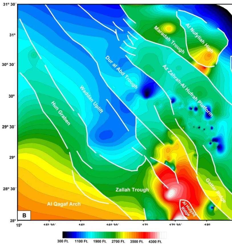
Fig. 5.6 Isopach and structural thickness map of Eocene time for the study area. Left hand images represent the thickness maps and white bold line appears as synclines represent the thickest trend in the area during that time. Right hand images represent the thickness maps integrated with main tectonic elements of the Sirt Basin and the white bold lines represent the major faults (after Mouzughi, and Taleb1981).
