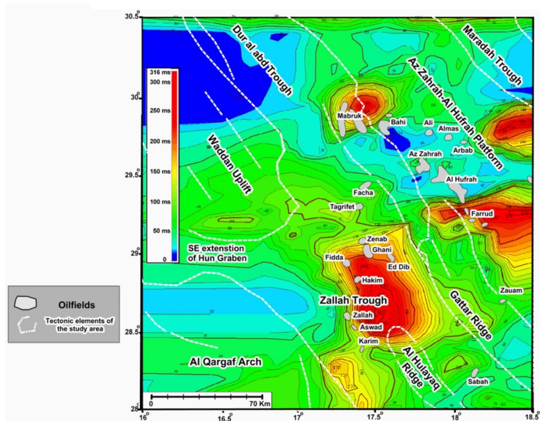
Fig. 6.21 The near top Harash to near top Zalten isochron contour
