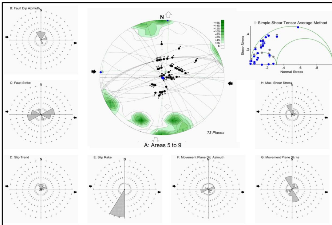
Fig. 7.14 Results of different stress phases for northwest Libya (Jifarah Basin and Nafusah Uplift). Field data diagram are Schmidt's projections of lower hemisphere. A: areas 5 to 9. Faults are great circles, slickenside lineations are dots with arrows indicating the sense of motion of the hanging wall. Computed stress axes are represented as large blue dot ( \sigma_1 ), medium blue dot ( \sigma_2 ) and small blue dot ( \sigma_3 ). Large divergent white arrows indicate the horizontal extensional stress direction ( \sigma_3 ) whilst large convergent black arrows indicate maximum principal stress axis ( \sigma_1 ). Rose diagrams for the structures observed northwest Libya (Jifarah Basin and Nafusah Uplift). The radius of the rose corresponds to the class with the highest frequency as represented in the figure (B to I).
