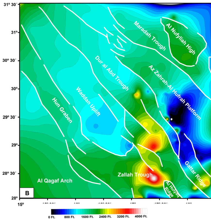
Fig. 5.4 Isopach and structural thickness map of Upper Cretaceous time for the study area. Left hand images represent the thickness maps and white bold line appears as synclines represent the thickest trend in the area during that time. Right hand images represent the thickness maps integrated with main tectonic elements of the Sirt Basin and the white bold lines represent the major faults (after Mouzoughi, and Taleb1981).
