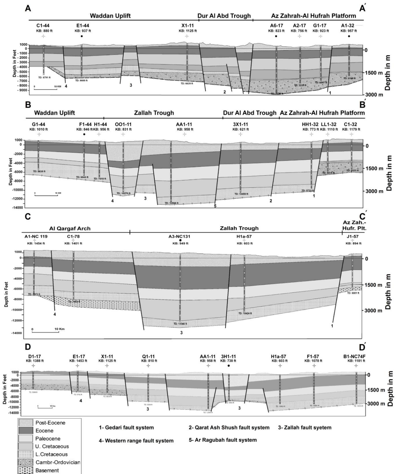
Fig. 8.2 Geological cross sections through the Zallah-Dur Al Abd Trough constrained by well data showing the tectonic evolution of the study area. Note the numerous faults, with only the larger ones shown here, demonstrating the distributed nature of deformation in the trough. Dramatic thickening of the Upper Cretaceous strata indicates that the rifting was most active at this time, followed by a period of Paleocene downwarping subsidence. For location see Fig. 8.1. Cross-sections labelled as aa', bb', and cc' were constructed perpendicular to the main structural elements of the study area with same horizontal scale, and are displayed with different vertical exaggeration whilst dd' oriented parallel to the boundary fault (longitudinal section).
