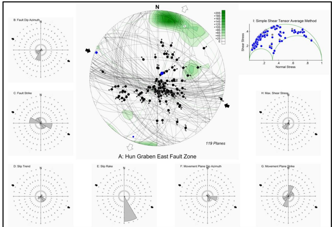
Fig. 7.7 Results of different stress phases for the Eastern Fault Zone (EFZ) of Hun Graben. Field data diagram are Schmidt's projections of lower hemisphere. A: Left Normal strike-slip faults. Faults are great circles, slickenside lineations are dots with arrows indicating the sense of motion of the hanging wall. Computed stress axes are represented as large blue dot ( \sigma_1 ), medium blue dot ( \sigma_2 ) and small blue dot ( \sigma_3 ). Large divergent white arrows indicate the horizontal extensional stress direction ( \sigma_3 ) whilst large convergent black arrows indicate maximum principal stress axis ( \sigma_1 ). Rose diagrams for the structures observed Hun Graben. The radius of the rose corresponds to the class with the highest frequency as represented in the figure (B to I).
