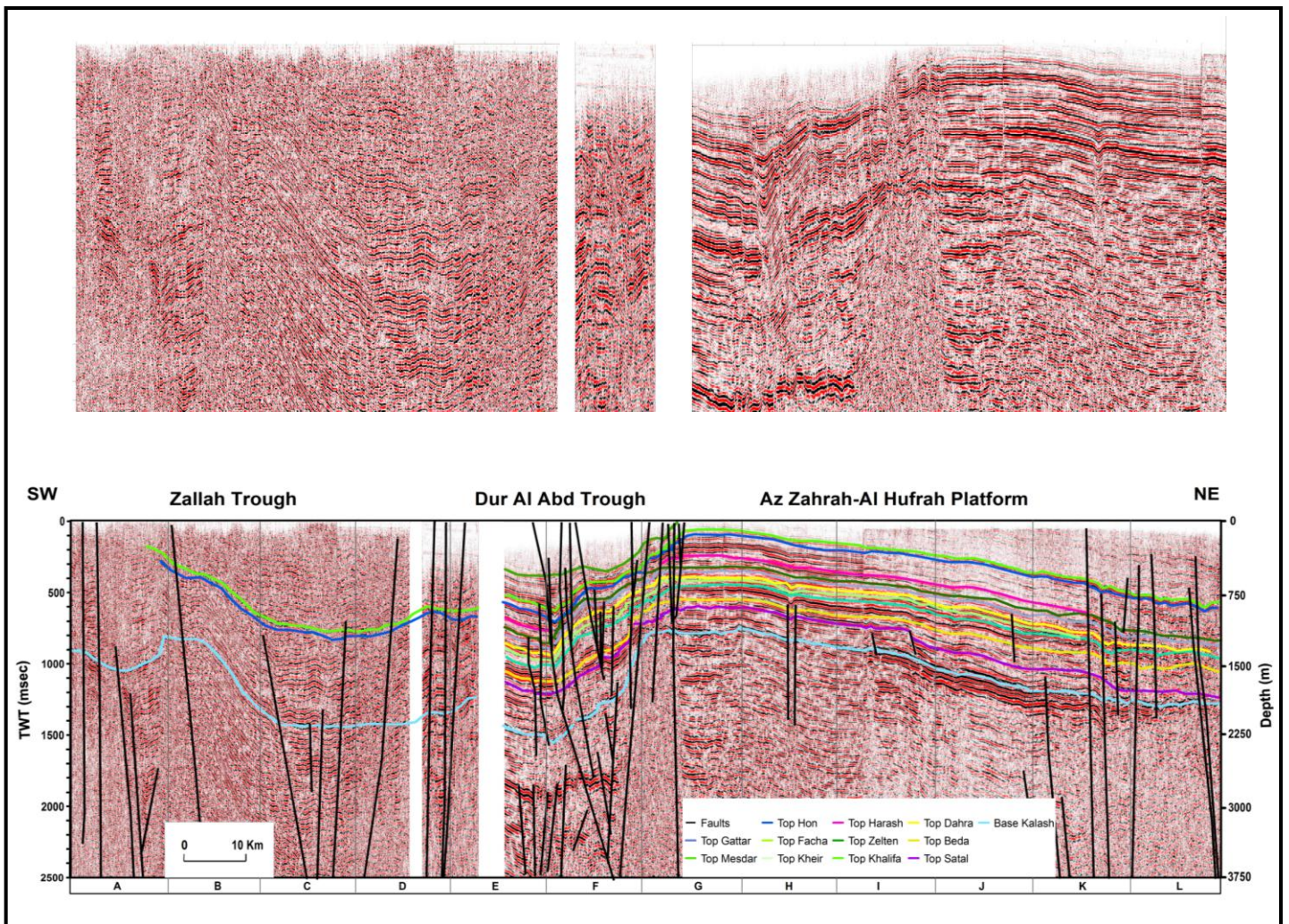
Fig. 6.8 Seismic cross section B-B' view of present day structure across the study area from the southwest to the northeast (See figure 1.4 for location).
