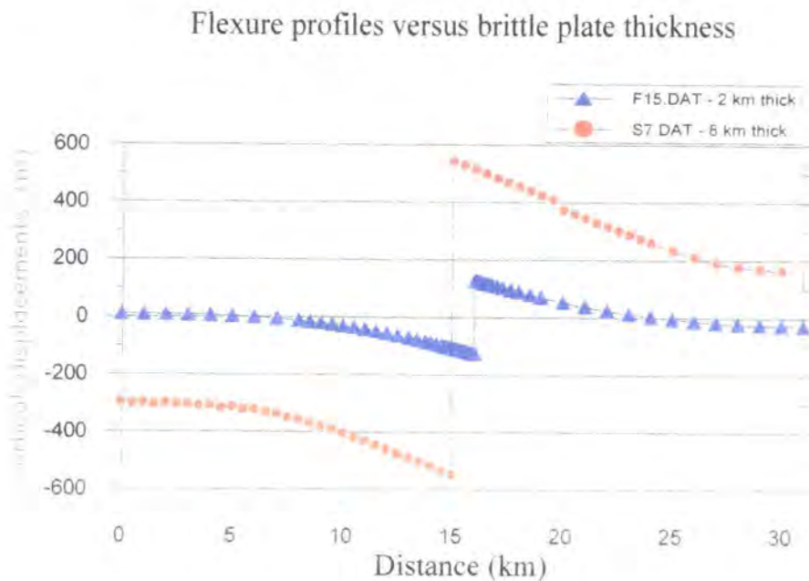
Fig. 5.9 Flexure profile versus brittle layer thickness, for model F* at maximum applied extension (model 2 km thick, 63° fault, 150 m of stretching) and model S* at maximum applied extension (model 8 km thick, 63° fault, 700 m of stretching). The fault throw and the plate curvature are greater for the thicker brittle layer.
