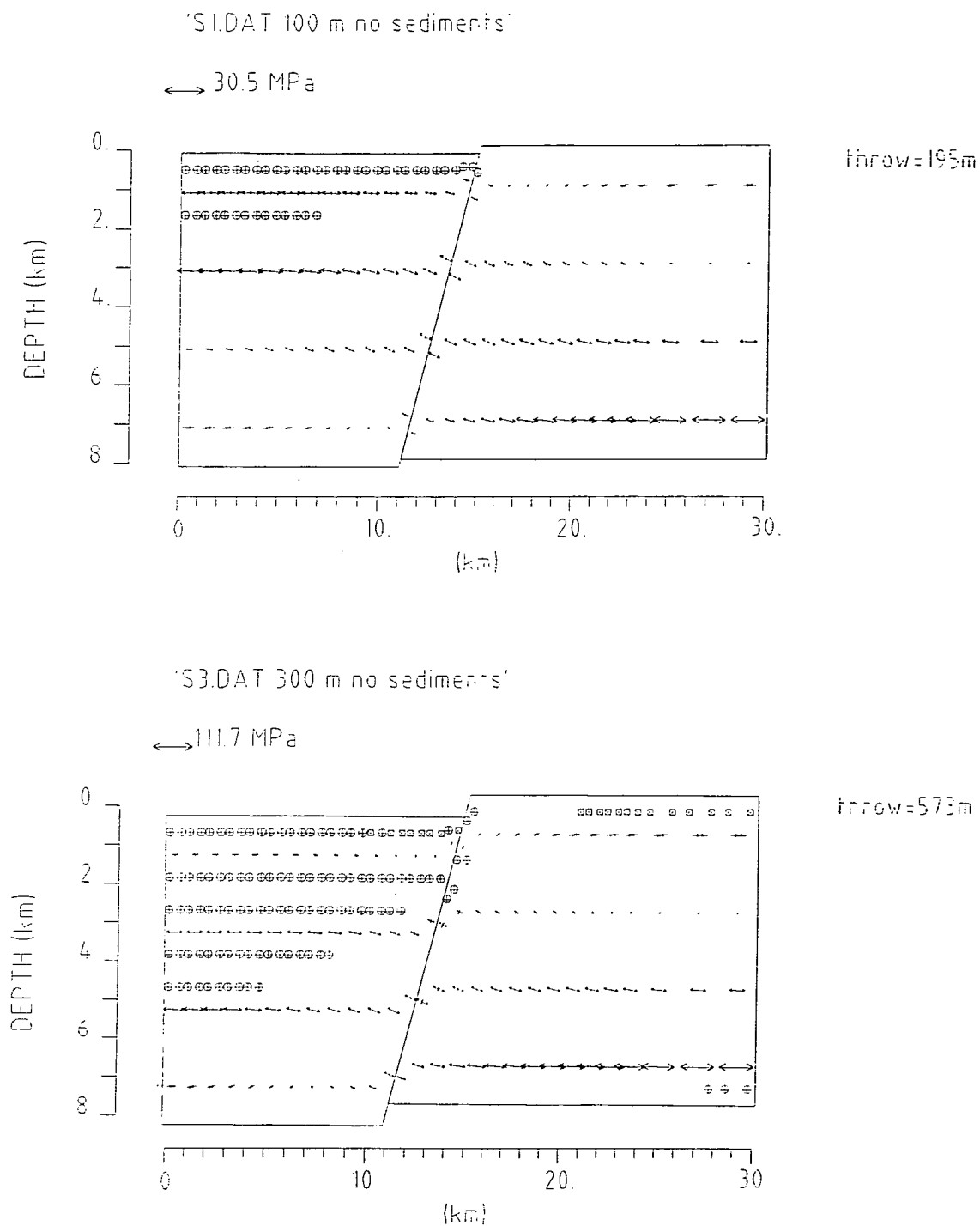
Fig. 5.4 Stress and failure pattern of model S* (8 km thick, 63° fault). The * denotes the number of 100 m increments of applied extension. There is no loading by infill. The maximum stress is shown at the top and the fault throw is shown at the right of each model. All symbols are as described in figure 5.2.
