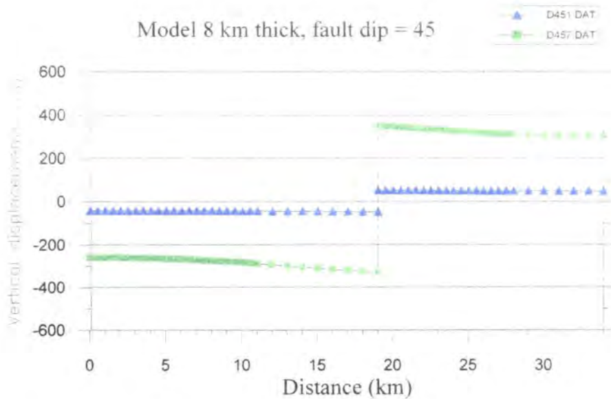
Fig. 5.8 The flexure profile of model D45* (8 km thick, 45^\circ fault) at 100 and 700 m of applied extension. The vertical displacements relative to the initial datum are greatly affected by the boundary conditions. The flexure profile is much nearer the horizontal than it should be for a longer or rotationally unconstrained model.
