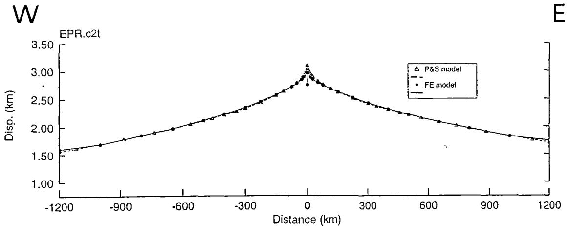
Fig. 4.3 The flexural profile of the finite element model EPR.C2T compared to the Parsons and Sclater (1977) predicted bathymetric profile. Model EPR.C2T is a normal subsidence model with an assumed compensation depth of 150 km. The viscoelastic relaxation time is 25000 yr.
