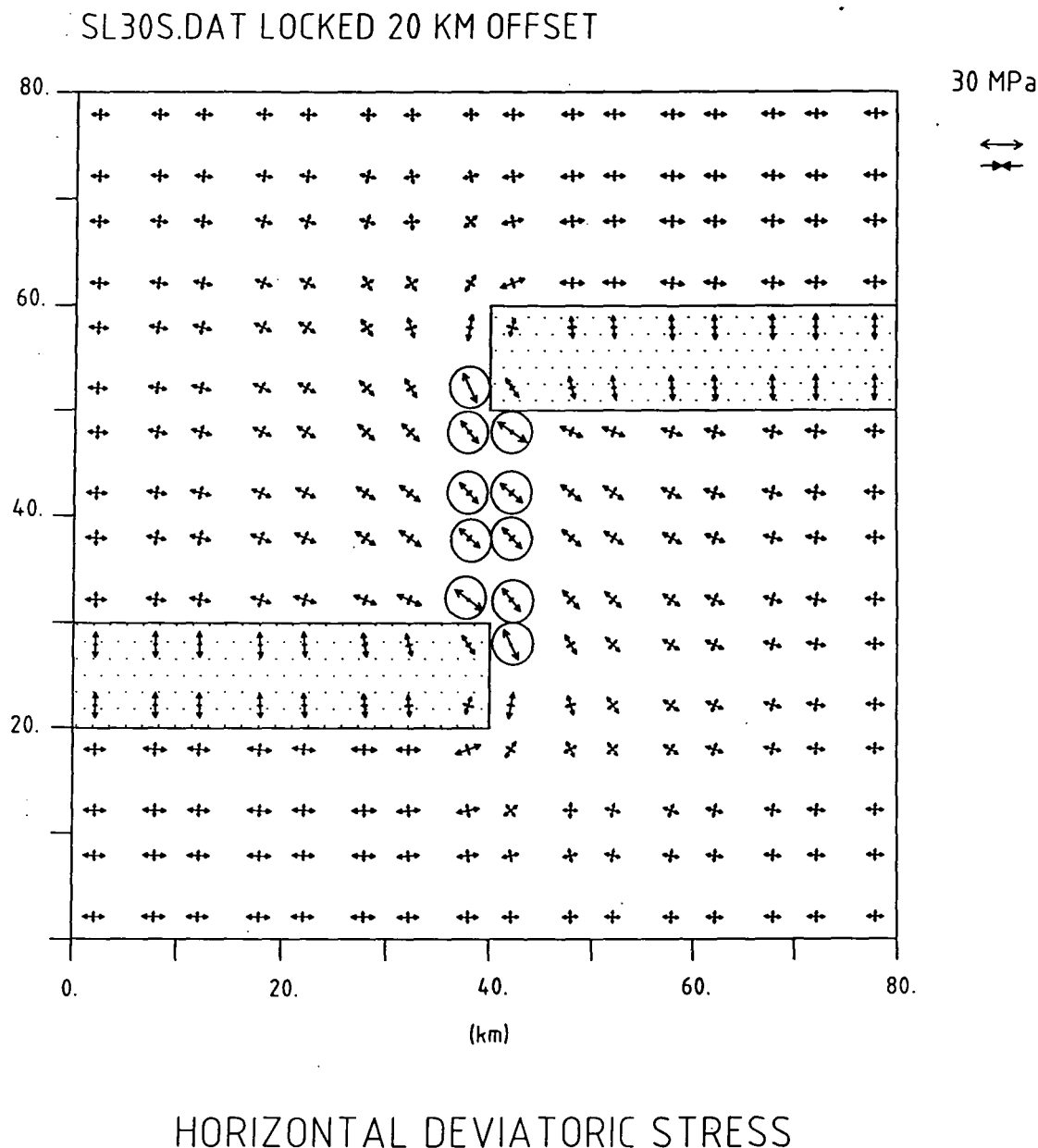
Fig. 6.20 Deviatoric stress pattern of model SL30S, which represents a 20 km non-transform offset between two slow spreading ridges. Rheologies and topographic loading are as in Fig. 6.13. The circles mark the regions where normal faults trending 35°-50° oblique to the ridge axis are predicted. Other symbols are as in Fig. 6.13. The deviatoric stress pattern is consistent with the 45° oblique basins and structural trends characteristics of some non-transform offsets.
