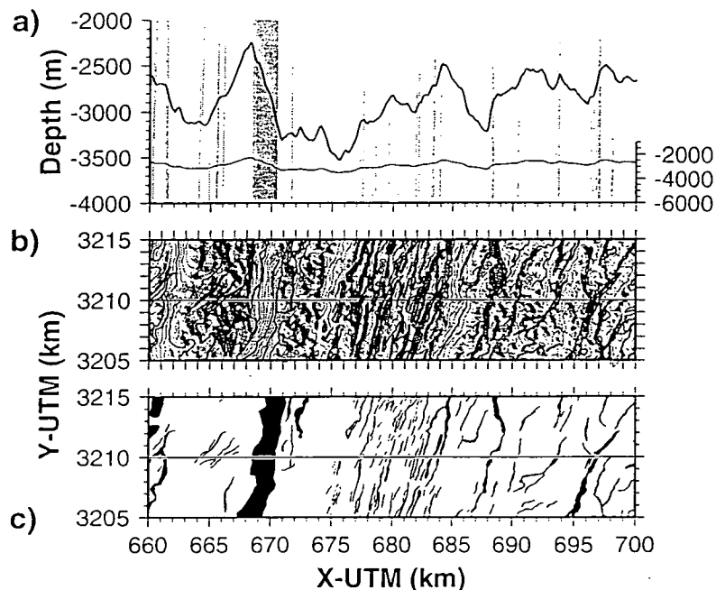
Fig. 1.5 Fault scarps across the MAR at 29^{\circ}N (segment centre). The bathymetric profile is shown with (8x) and no vertical exaggeration (thick and thin lines, respectively). (a) Comparison of the interpreted fault scarps (grey bars) from the backscatter data with multibeam bathymetric data. (b) Location of the bathymetric profile on a relief map of the area (100 m contours). (c) Faults interpreted from digital-side scan sonar mosaics (after Escartin et al., 1999).
