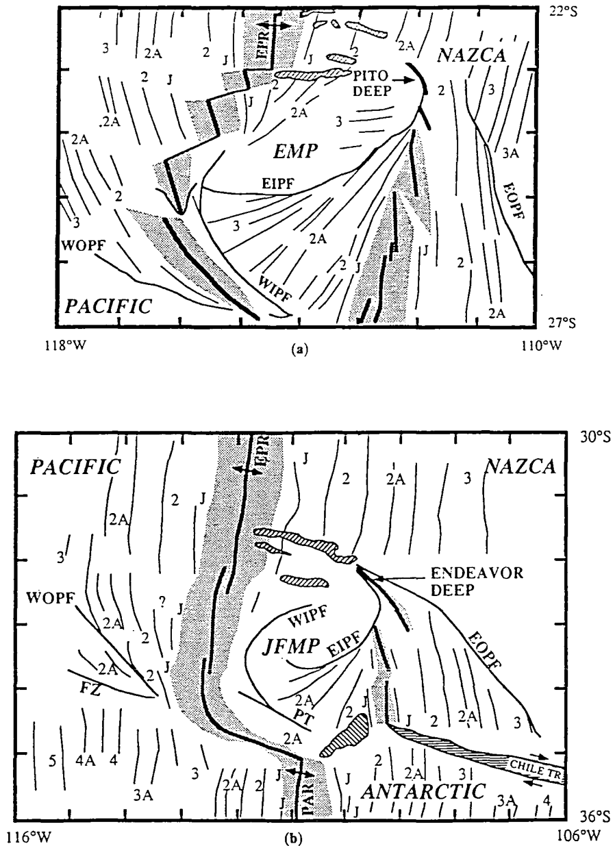
Fig. 1.9 Structures and isochrons of (a) Easter microplate (EMP) and (b) Juan Fernandez microplate (JFMP). Heavy lines indicate the spreading centres and medium lines are the pseudofaults (WOPF, WIPF, EOPF, EIPF are the western outer and inner and eastern outer and inner pseudofaults, respectively). Light lines and lettering are the magnetic isochrons. The stippled region represents the extent of the Brunhes anomaly. Diagonally hatched areas are the compressional ridges at the northern boundaries of the microplates, and complex structures of the JFMP-Antarctic boundary. Horizontal hatching is the Chile Transform. FZ indicates the inactive western limb of the Chile transform and PT is the part of Chile transform that has been inactivated by the growth of the Juan Fernandez microplate. EPR and PAR are the East Pacific Rise and Pacific-Antarctic Rise, respectively (after Searle et al., 1993).
