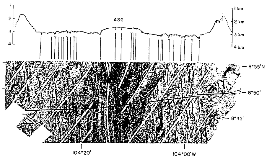
Fig. 1.4 Faults scarps across the East Pacific Rise at 8^{\circ}50'N . Location of the Deeptow bathymetric profile (at the top) is delineated on the seaMARC II side scan data (at the bottom) with a solid line. Identified fault scarps are indicated by thin lines below Deeptow profile and by arrows on seaMARC II data (after Carbotte and Macdonald, 1994).
