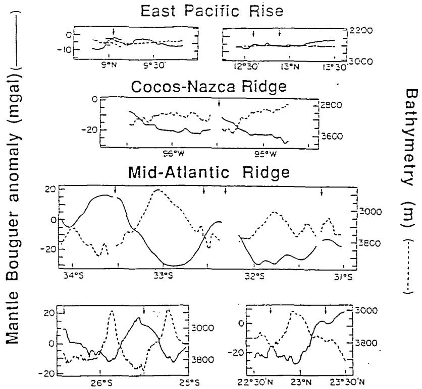
Fig. 1.2 Along-axis profiles of seafloor depth (dashed lines) and Mantle Bouguer Anomaly (solid lines) at fast, intermediate and slow spreading ridges. Arrows mark first and second order discontinuities (after Lin and Phipps Morgan, 1992).
