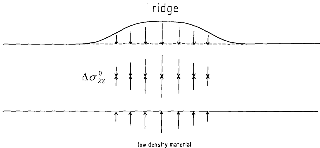
Fig. 6.2 The surface and subsurface loads associated with the topography of mid-ocean ridges produce vertical non-lithostatic stresses \Delta\sigma_{zz}^0 in the lithospheric plate.
