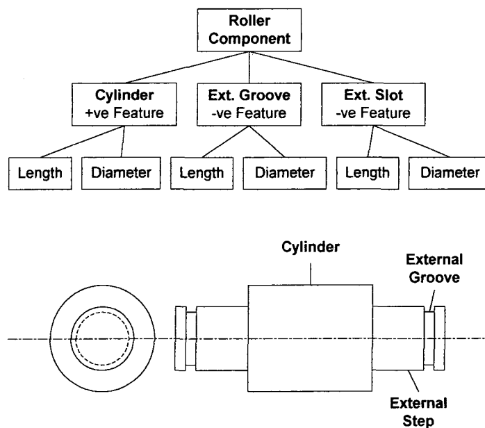
Figure 7-2: Roller Component
