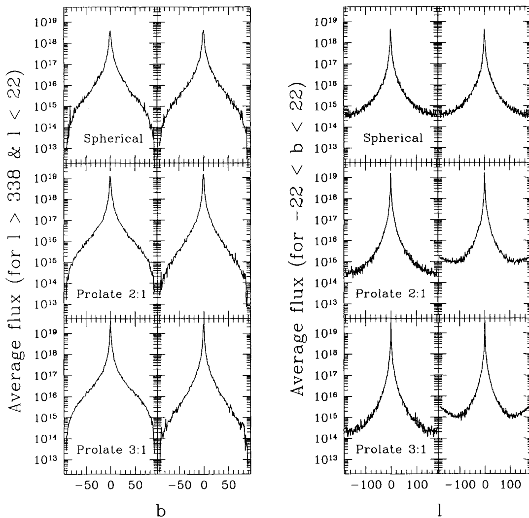
Figure 4.18: As in Figure 4.17 but for a prolate distribution of substructure halos.
