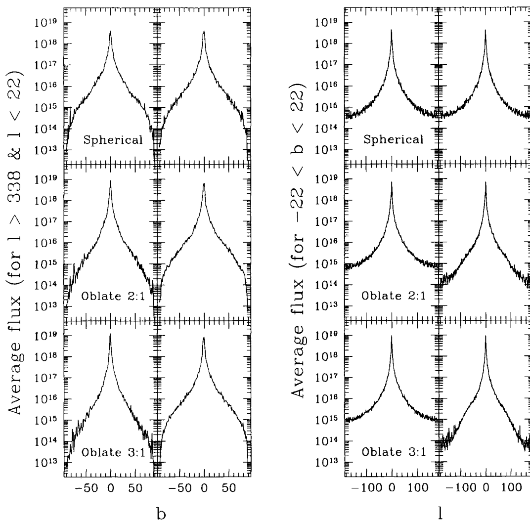
Figure 4.17: The effect of halo shape on the average gamma-ray flux from sub-halos. Substructure halos are randomly drawn from an oblate distribution with the indicated axis ratios. The left panels have the observer placed in the long axis whilst the right panels have the observer in the short axis.
