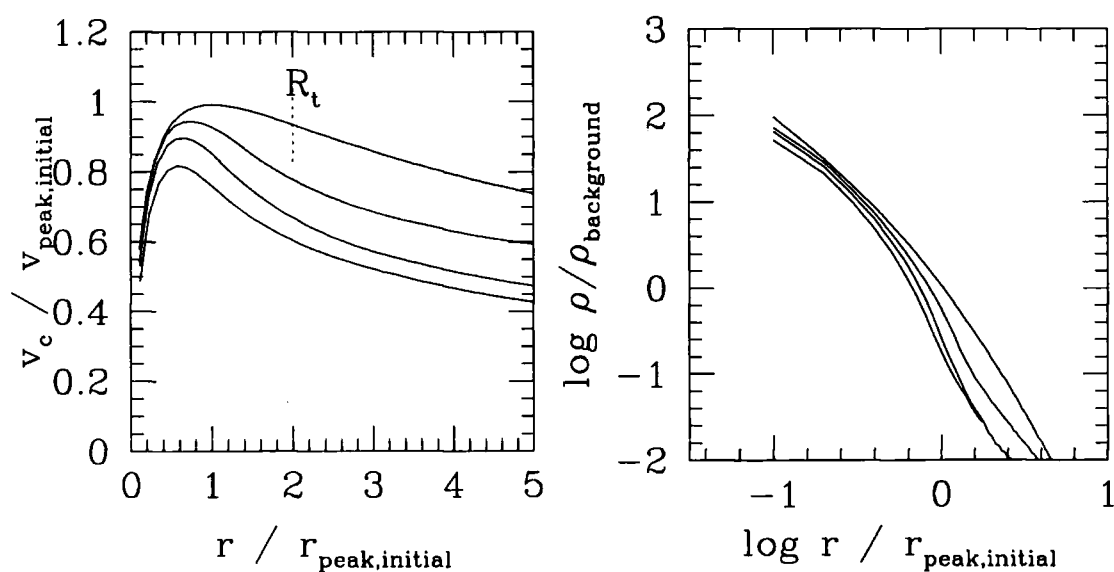
Figure 4.23: The evolution of the circular velocity and density profiles of the satellite moving on a circular orbit at 40 kpc from the center of a Galactic potential. The curves show the initial configuration and subsequent times of 1, 2 and 3 Gyrs.
