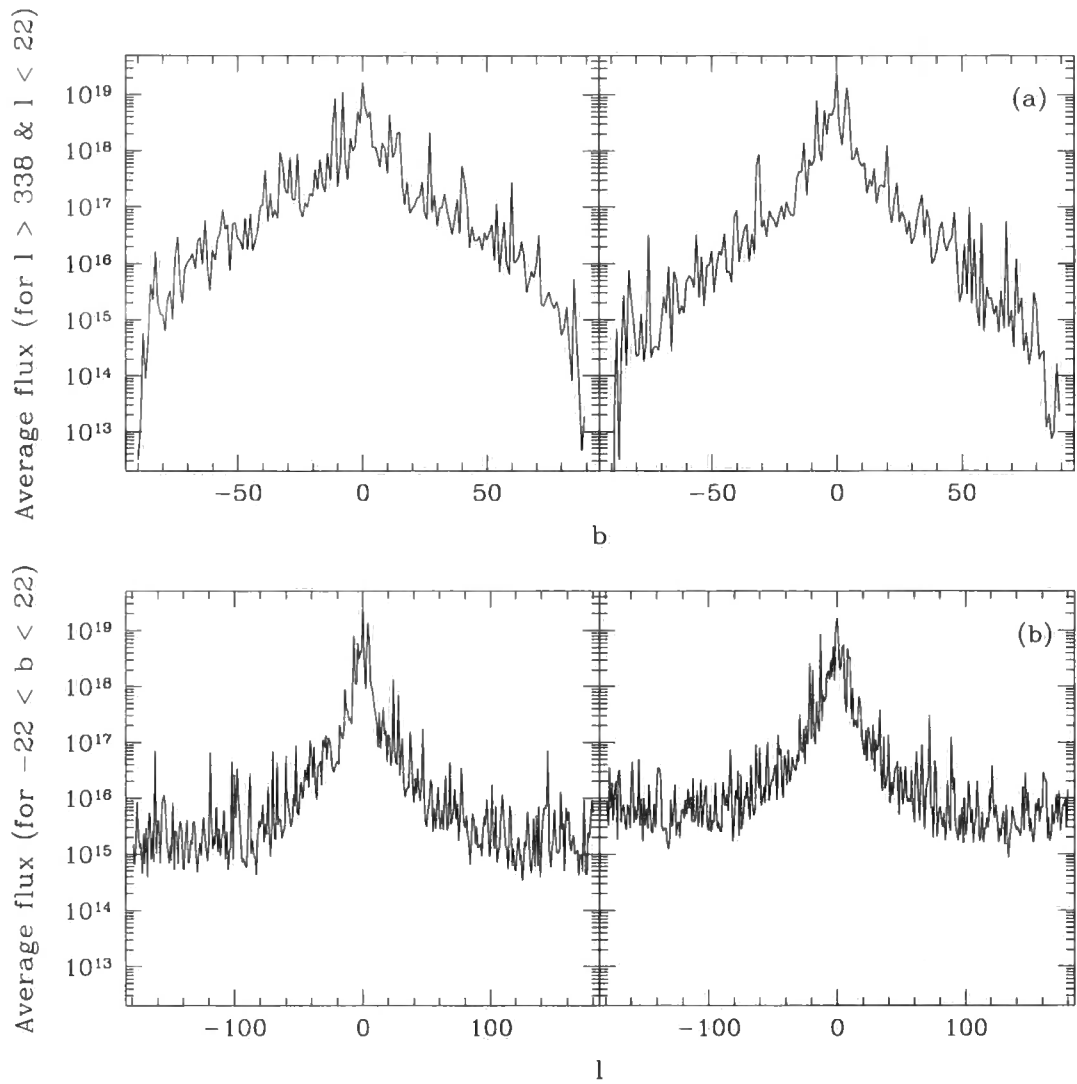
Figure 4.16: The average gamma-ray flux per square degree from dark matter substructure as measured along a great circle of constant galactic latitude (a) and longitude (b). The average has been taken over a strip of width 44 degrees and in both cases the left hand plot represents the view along the short axis while the right hand side is the view along the long axis.
