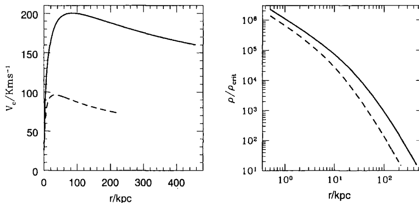
Figure 2.1: The rotation curves: V_c = \sqrt{GM/r} (left panels) and density profiles (right panels) for the two halo models discussed in the text. Solid lines correspond to the parent halo; dashed ones to the satellite.
