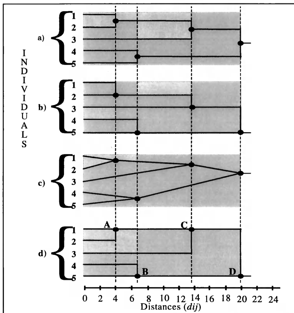
Figure 5.1 - Four different formats to represent dendrograms.
