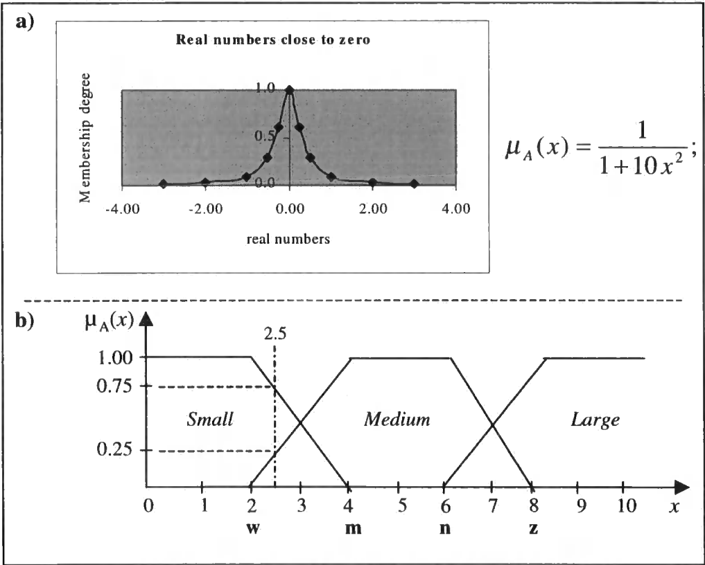
Figure 7.4 – Examples of Gaussian and Trapezoidal membership functions.
