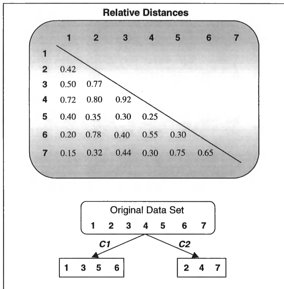
Figure 6.2 - Dissimilarity matrix and basic test data set
