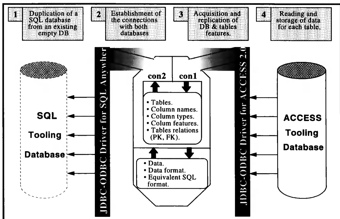
Figure 3.13 - Data translation process
