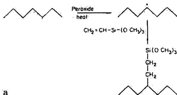
Fig. 2.12 (The peroxide heating into an extruder)
