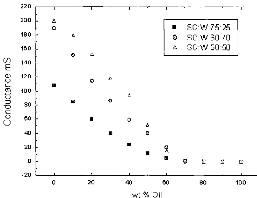
Figure 5.21 The effect of surfactant concentration on conductivity
