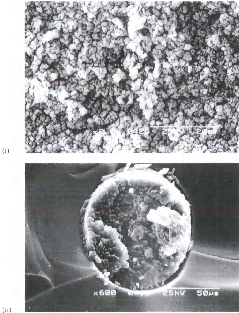
Figure 4.3 SEM images of the fractured surface of (i) a monolith prepared from MMA, EGDMA, DDAB and water and (ii) the resulting filled capillary (appendix A4)
