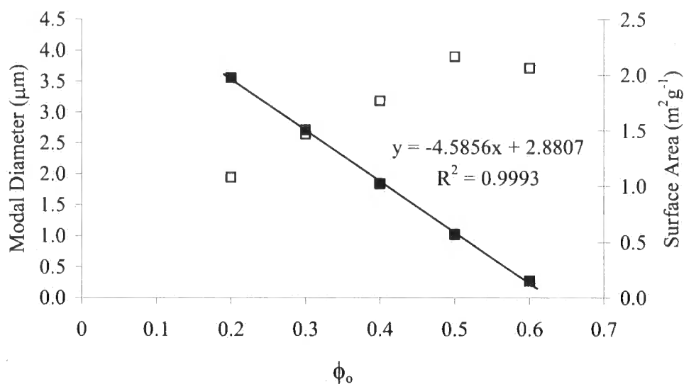
Figure 5.14 Modal pore diameter ( \square ) and surface area ( \blacksquare ) against oil fraction, \phi_o . The remaining fraction consists of SDS, 1-propanol and water in a 20:40:40 ratio. The error bars are smaller than the data points.
