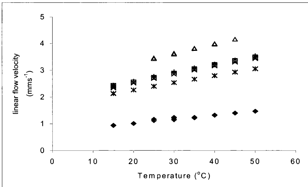
Figure 6.18 The effect of temperature on linear velocity in monolithic columns 1-4 (+, *, \square , x) and 11 ( \Delta ) and an ODS packed column ( \blacklozenge ).
