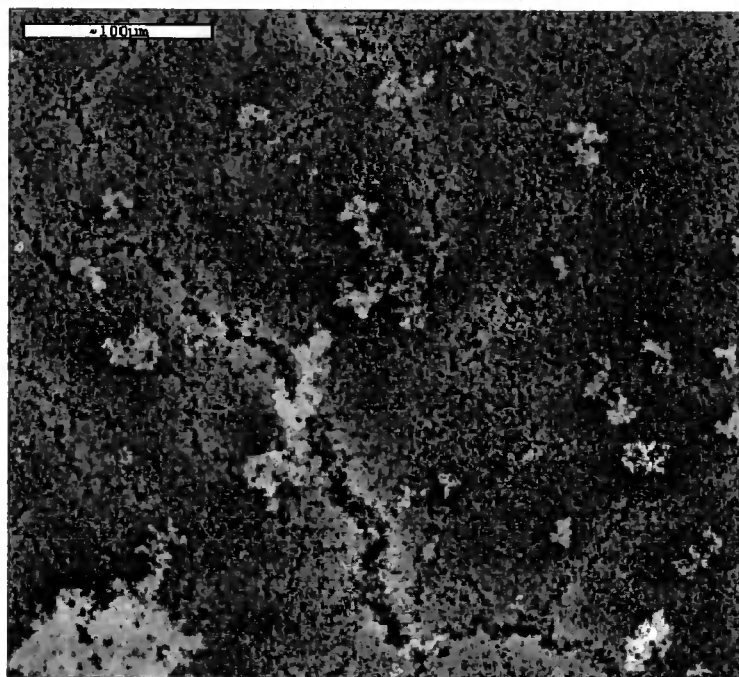
Figure 4.14 SEM images of monolith prepared with (i) a layer of heptane on the surface; (ii) an air, microemulsion interface.
