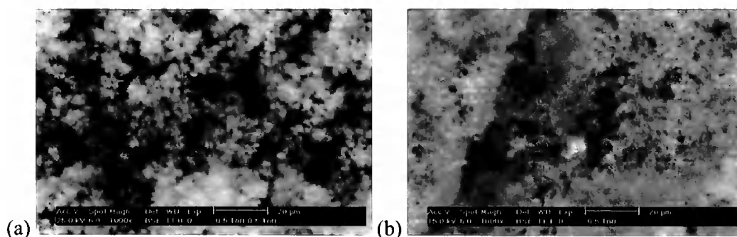
Figure 5.32 SEM images (1000X magnification) of a monolith prepared with an \text{SDS}_{(aq)} ;1-propanol ratio of 60:40 wt/wt containing 20 wt% oil. (a) fractured surface and (b) air-microemulsion surface.
