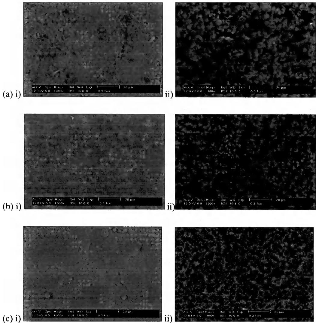
Figure 5.12 SEM images (1000X magnification) of the monolith surface polymerised in contact with air (i) and the fractured section (ii) of monoliths prepared from (a) 50.0 wt% oil, 20.0 wt% water, 10.0 wt% SDS, 20.0 wt% 1-propanol; (b) 60.0 wt% oil, 16.0 wt% water, 8.0 wt% SDS, 16.0 wt% 1-propanol; (c) 50.0 wt% oil, 10.0 wt% water, 13.3 wt% SDS, 26.7 wt% 1-propanol
