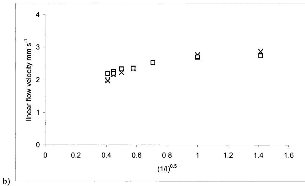
Figure 6.10 The effect of buffer ionic strength on linear velocity in a) an ODS packed column; b) a porous monolith filled column at 50 % MeCN v/v and × contains 0.3 wt% AMPS, □ contains 0.6 wt% AMPS.
