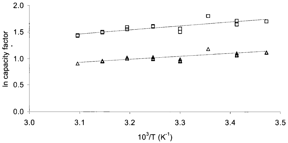
Figure 6.17 Van't Hoff plot for Hypersil ODS column for dipropylphthalate ( \Delta ) and diphenylphthalate ( \square ).
