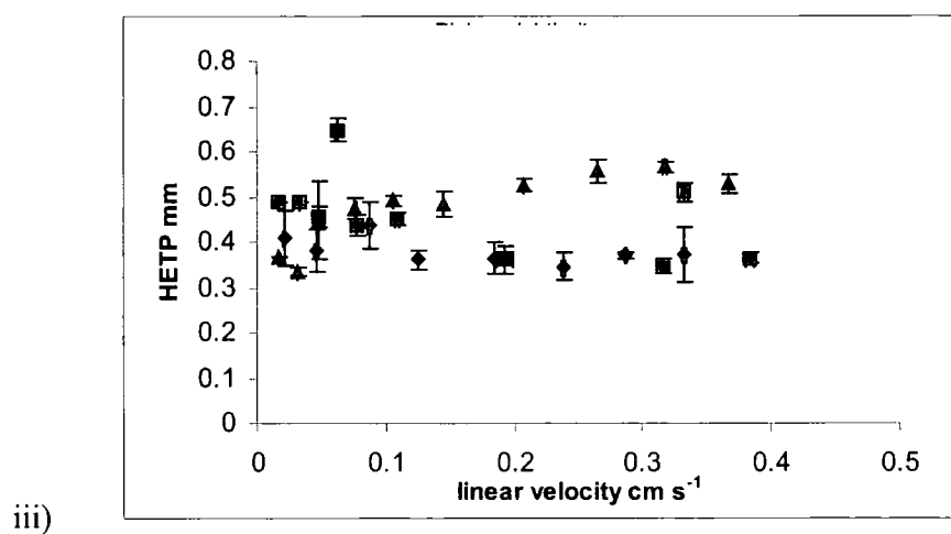
Figure 6.13 Van Deemter plots for (i) thiourea; (ii) dipropylphthalate; and (iii) diphenylphthalate on 4.9 (◆), 5.3 (■) and 5.8 (▲) μm monoliths.
