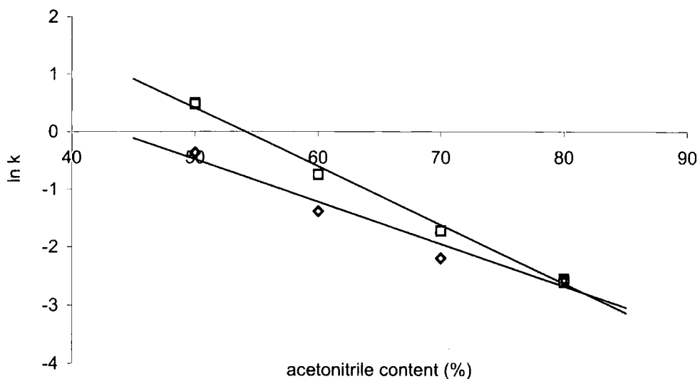
Figure 6.4 Effect of acetonitrile content of the mobile phase on the logarithm of the capacity factor, k , of dipropylphthalate ( \diamond ) and diphenylphthalate ( \square ) on a 3.3\mu\text{m} monolithic stationary phase (Table 6.1.5).
