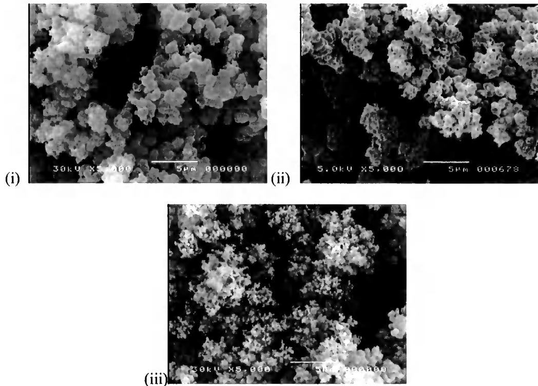
Figure 4.11 SEM images of monoliths prepared from microemulsions containing (i) 50.8 wt% oil, 39.5 wt% water, 9.7 wt% SDS (appendix A10); (ii) 41.0 wt% oil, 39.4 wt% water, 19.6 wt% SDS (appendix A9); (iii) 31.0 wt% oil, 39.4 wt% water, 29.6 wt% SDS (appendix A11).
