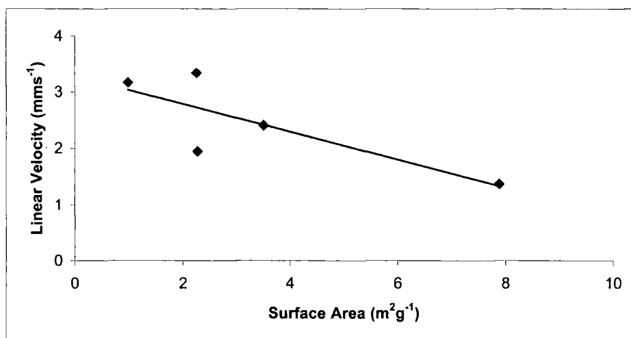
Figure 6.9 Effect of surface area on EOF for monolithic stationary phases prepared using BMA and EGDMA (60:40 w/w).
