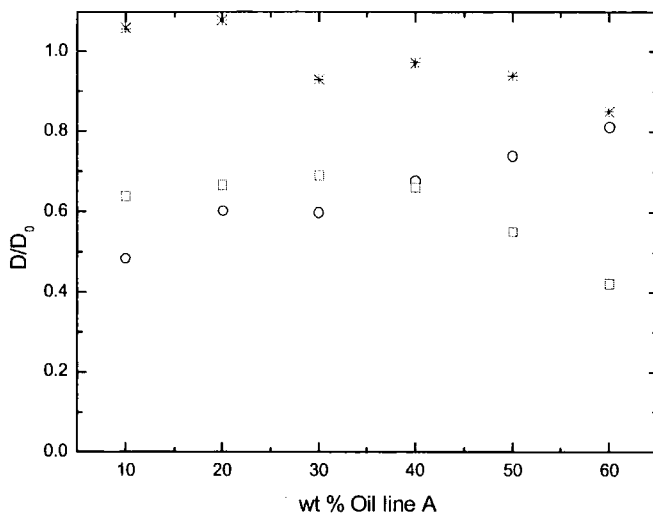
Figure 5.36 Normalised diffusion of surfactant (□), water (*) and oil (○) represented by points along line A in Figure 5.4.
