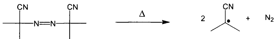
Figure 4.7 Thermal decomposition of AIBN
