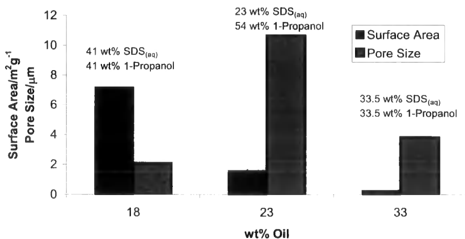
Figure 5.23 The pore size and surface area of monoliths prepared from microemulsions in appendix C 4 – 7. Error bars are obscured by the data bar borders.
