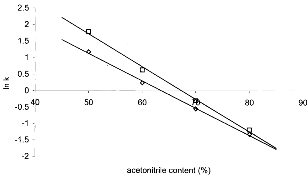
Figure 6.5 Effect of acetonitrile content of the mobile phase on the logarithm of the capacity factor, k , of dipropylphthalate ( \diamond ) and diphenylphthalate ( \square ) on 3\mu\text{m} ODS packing.
