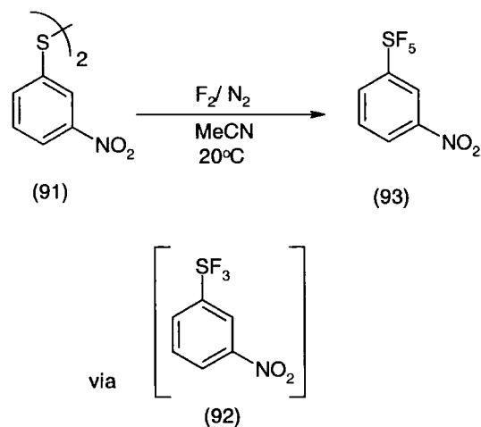
Fig 6.6: One-step fluorination
