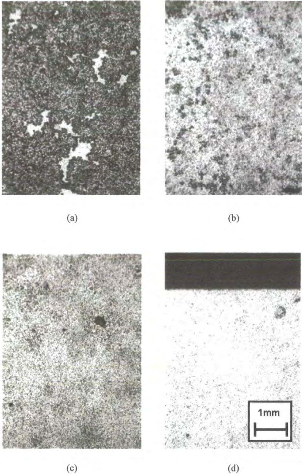
Figure 6.25 Optical micrographs ( \times 20 magnification) of the surface of the Al electrode following a constant stress (current density = 15 \text{ mA cm}^{-2} ) applied for 25 minutes. Photographs correspond to devices processed in different ways before the deposition of the Al top electrode: (a) untreated; (b) dried for 12 h in high vacuum; (c) annealed for 12 h at 35 \text{ }^\circ\text{C} in high vacuum; and (d) annealed for 12 h at 60 \text{ }^\circ\text{C} in high vacuum.
