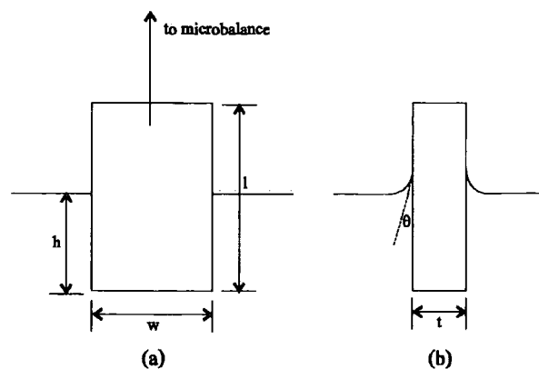
Figure 4.5 A Wilhelmy plate: (a) front view, (b) side view.
