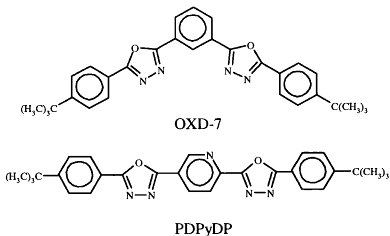
Figure 7.8 Molecular structures of OXD-7 and PDPyDP.
