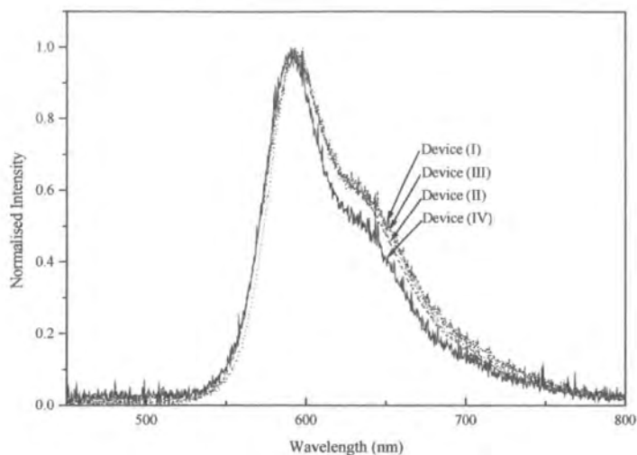
Figure 7.23 EL spectra of the LEDs.
