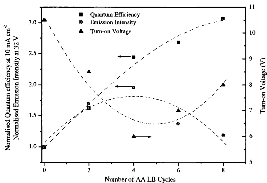
Figure 6.6 The trend of quantum efficiency, emission intensity and turn-on voltage for the device with different AA LB cycles.
