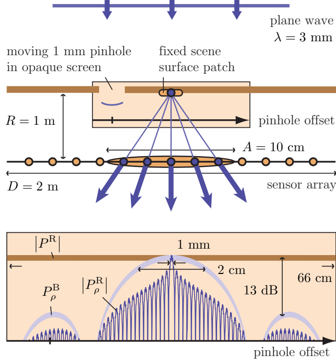
Figure 6: Images of nearby objects formed from pure quasi light fields are blurry. In the scene, a small backlit pinhole moves across the field of view of a sensor array that implements three cameras, each computing one pixel value for each pinhole position, corresponding to a fixed surface patch. As the pinhole crosses the fixed scene surface patch, the near-zone camera resolves the pinhole down to its actual size of 1 mm, while the far-zone camera records a blur 66 cm wide.
