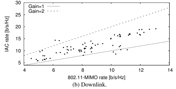
Figure 13: 3-clients and 3-APs. The figure shows a scatter plot of the rate under IAC and 802.11-MIMO, for 3-client and 3-AP scenarios. The two lines are for reference; they illustrate the cases of no-gain in transfer rate, i.e., “Gain=1” and a doubling of transfer rate, i.e., “Gain=2”. The results show that, on average, IAC increases the rate by 1.8x on the uplink and 1.4x on the downlink.
