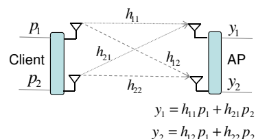
Figure 1: Throughput of current MIMO LANs is limited by the number of antennas per AP. The h_{ij} 's are known channel coefficients, and the p_i 's are concurrent packets. The client transmits two concurrent packets. The AP receives a different linear combination of the transmitted packets on each antenna, which it solves to obtain the packets.
