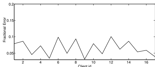
Figure 16: Channel Reciprocity. This figure plots the fractional difference between the direct estimate of a downlink channel and its estimate based on reciprocity. The x-axis refers to runs at different clients/locations. The figure shows that estimates based on reciprocity provide a reasonable accuracy and can be used in IAC.
