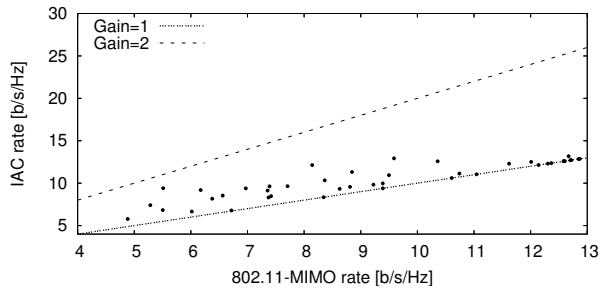
Figure 14: 1-client and 2-APs. The figure shows that IAC is beneficial even when the network has one active client. In this case, IAC provides a diversity gain over 802.11-MIMO because it allows the client to choose between downloading two concurrent packets from one of the two APs, or using both APs concurrently, downloading one packet from each.
