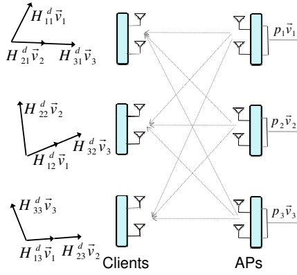
Figure 6: Three Packets on the Downlink. The APs deliver one packet to each client. To enable the client to decode its packet, all the undesired packets at the client must be aligned.
