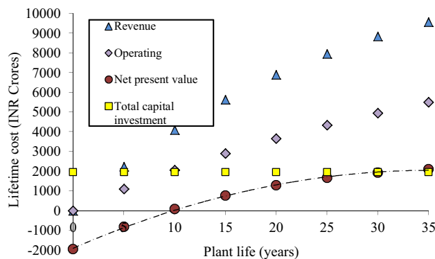
Fig. 8 Effect of plant life on total capital investment, total operating cost, total revenue and net present value; plant load = 210 MW
