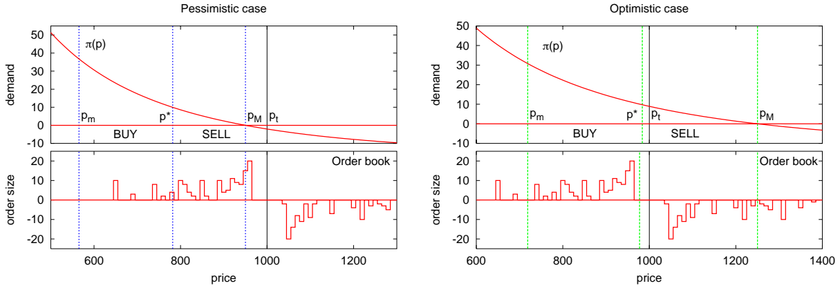
Figure 9: (Left) The role of the CARA demand function (5) in the order placement decision when p_M = \hat{p}_{t+\tau}^i < p_t and for a given snapshot of the book. (Right) The role of the CARA demand function (5) in the order placement decision when p_M = \hat{p}_{t+\tau}^i > p_t and for a given snapshot of the book. The figures at the bottom show a typical pattern of the limit order book at a given time in a simulation. Buy orders placed in the book are represented as positive volume, while sell orders placed in the book are represented as negative volume. The top figures are particular instances of Figure 1. The intersections determine the three different price levels p_m , p^* and p_M for the case of optimistic trader ( p_M > p_t ) (right) and pessimistic trader ( p_M < p_t ) (left).
