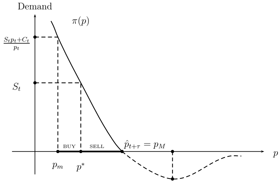
Figure 1: Determination of the buy/sell price range of a typical agent (the superscript i has been suppressed here). The curve labelled \pi(p) graphs Eq. (8) with the dashed section representing negative (short position) demand. The upper limit of the price range is p_M where the positive (long position) demand comes to zero. The minimum limit p_m is determined by the agent's current wealth holding. The price p^* that separates the buy/sell regions is determined by the agent's current holding, S_t , of stock.
