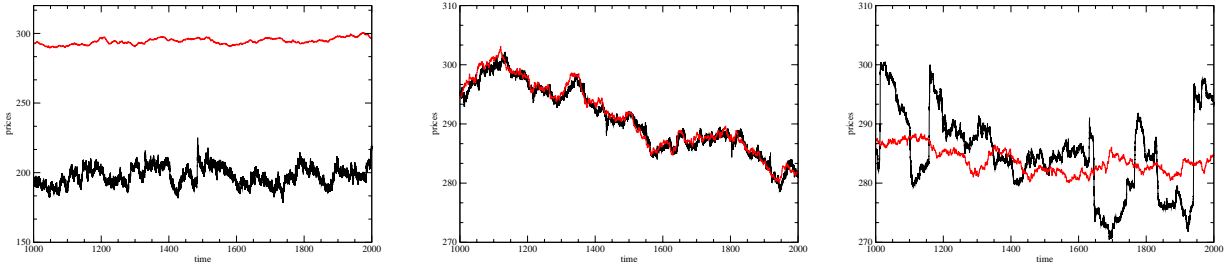
Figure 2: Price (black) and fundamental value (red) with only noise trading (left, \sigma_1 = 0.00 , \sigma_2 = 0.00 ), noise trading and fundamentalism (center, \sigma_1 = 10.00 , \sigma_2 = 0.00 ) and noise trading, fundamentalism and chartism (right, \sigma_1 = 10.00 , \sigma_2 = 1.20 ).
