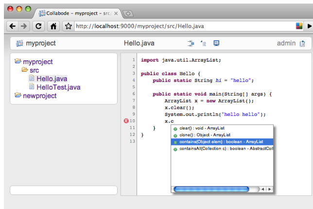
Figure 1: The Collabode web-based IDE allows multiple simultaneous editors to work together.
