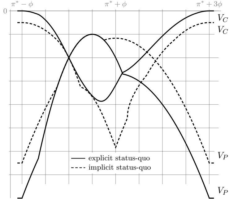
Figure 1.5: Equilibrium value functions \pi^* = 2, \phi = 1, \delta = 0.5, r_d = 0.5
