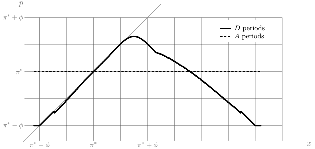
Figure 1.2: Equilibrium policy with explicit status-quo \pi^* = 2 , \phi = 1 , \delta = 0.5 , r_d = 0.5
