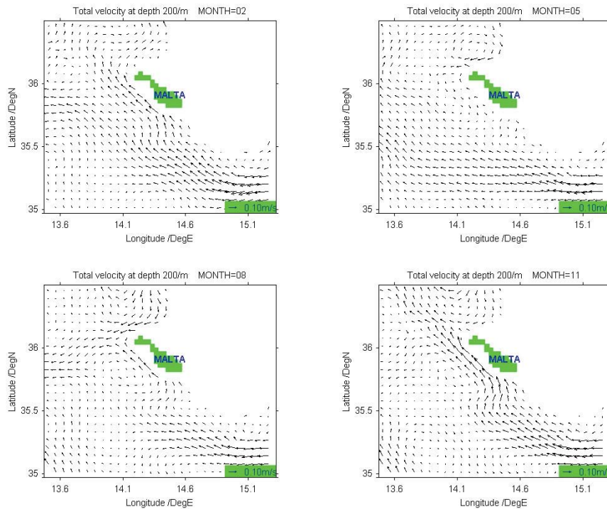
Figure 37. Field of velocity at 200m depth. The stable currents at the edge of the shelf support the hypothesis of a vertical movement of LIW over the outer shelf, which could enhance the biological productivity south of the Maltese Islands. These currents could also contribute to the dispersal of hake and deep water pink shrimp eggs and larvae produced by spawners over the outer shelf–upper slope, west of the Maltese Islands.
