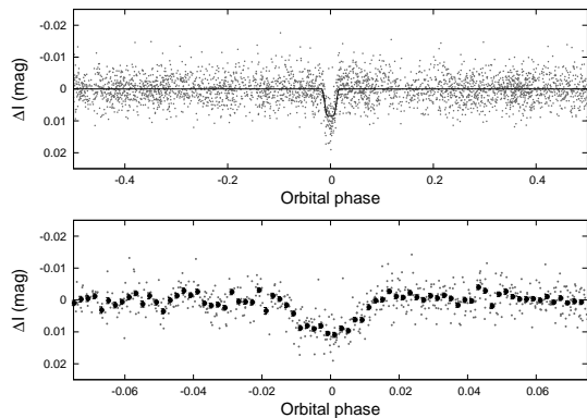
FIG. 1.— Unbinned light curve of HAT-P-30, including \approx 3200 data points obtained with the HAT-5 and HAT-9 telescopes of HATNet in the instrumental I_C band with a 5.5-minute cadence (see the text for details). The data have been folded with the period P = 2.8105951 days resulting from the global fit described in Section 3). The solid line shows a simplified transit model fit to the light curve (Section 3.2). The bottom panel shows a zoomed-in view of the transit, the filled circles show the light curve binned in phase with a bin-size of 0.002.
