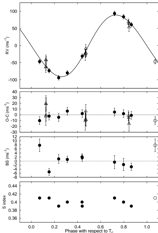
FIG. 2.— Top panel: Keck/HIRES RV measurements (filled circles) and Subaru/HDS RV measurements (open triangles) for HAT-P-30 shown as a function of orbital phase, along with our best-fit model (see Table 4). Zero phase corresponds to the time of mid-transit. The center-of-mass velocity has been subtracted. Second panel: Velocity O-C residuals from the best fit. The error bars include a component from astrophysical/instrumental jitter ( 6.3 \text{ m s}^{-1} for HIRES and 2.1 \text{ m s}^{-1} for HDS) added in quadrature to the formal errors such that \chi_p^2 = 1 (see Section 3.2). Third panel: Bisector spans (BS) for the HIRES spectra, with the mean value subtracted, and the measurement from the template spectrum is included. Bottom panel: Chromospheric activity index S measured from the Keck spectra. Note the different vertical scales of the panels. Observations shown twice are represented with open circles.
