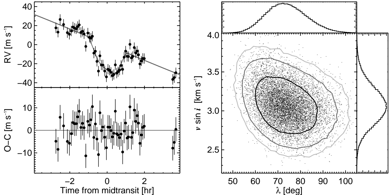
FIG. 4.— Rossiter-McLaughlin effect for HAT-P-30 Left .—Apparent radial velocity variation on the night of 2011 Feb 21, spanning a transit. The top panel shows the observed RVs. The bottom panel shows the residuals between the data and the best-fitting model. Right .—Joint constraints on \lambda and v \sin i_* . The contours represent 68.3%, 95.4%, and 99.73% confidence limits. The marginalized posterior probability distributions are shown on the sides of the contour plot.
