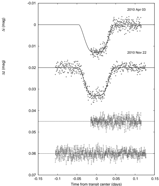
FIG. 3.— Unbinned instrumental i band and z band transit light curves, acquired with KeplerCam at the FLWO 1.2 m telescope. The light curves are displaced vertically for clarity. Our best fit from the global modeling described in Section 3.2 is shown by the solid lines. Residuals from the fits are displayed at the bottom, in the same order as the top curves.
