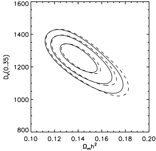
Figure A2. Comparison of the LRG-only likelihood surface computed with the analytic approximation of P_{\text{nw}} in Eqn. 29 of Eisenstein & Hu (1998) (solid, as in Fig. 5) compared with the result when using the b-spline fit described in Appendix A3 (dashed).
