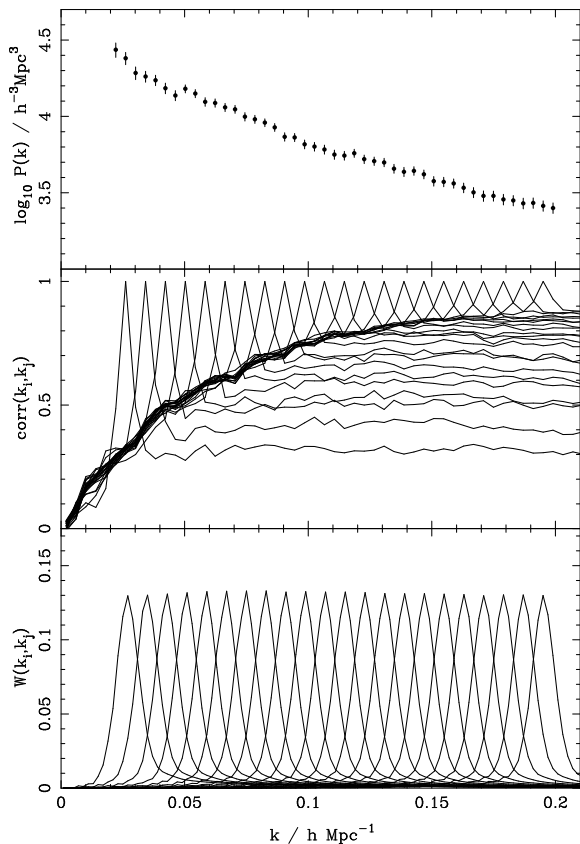
Figure 2. Top panel: Measured \hat{P}_{halo}(k) bandpowers. Error bars indicate \sqrt{C_{ii}} (Eq. 3). Middle panel: Correlations between data values calculated using Log-normal catalogues, assuming our fiducial cosmological model. Bottom panel: The normalized window function for each of our binned power spectrum values with 0.02 < k < 0.2 h Mpc ^{-1} . Each curve shows the relative contribution from the underlying power spectrum as a function of k to the measured power spectrum data. The normalisation is such that the area under each curve is unity. For clarity we only plot curves for every other band power.
