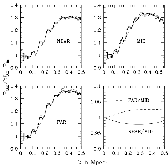
Figure 4. BAO-damping times polynomial fits to P_{halo}(k, \mathbf{p}_{fid})/P_{lin}(k, \mathbf{p}_{fid}) for our mock NEAR, MID, and FAR LRG reconstructed halo density field subsamples in Reid et al. (2008); \{z_{NEAR}, z_{MID}, z_{FAR}\} = \{0.235, 0.342, 0.421\} . The smooth component of these fits (dashed curves) enter our model P_{halo}(k, \mathbf{p}) through Eqns. (14), while the amplitude of the BAO suppression \sigma_{halo}^2 enters in Eqn. 10. Lower right panel: Ratio of the shape of the smooth components for the NEAR and FAR redshift subsamples to the MID redshift subsample.
