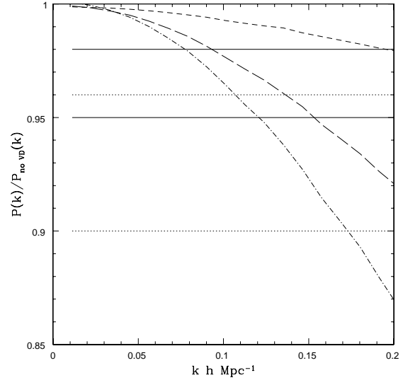
Figure B1. We compare three models including central galaxy velocity dispersion to our fiducial model with no central galaxy velocity dispersion ( f_{cen, err} = b_{vel} = 0 ) by showing the ratio of P_{halo}(k, \mathbf{p}_{fid}) for the models. The dashed curve has f_{cen, err} = 0.2 , b_{vel} = 0 (‘optimistic’); the long dashed curve has f_{cen, err} = 0.4 , b_{vel} = 0 (‘conservative’); the dash-dot curve has f_{cen, err} = 0.2 , b_{vel} = 0.6 (‘extreme’). The straight lines show our fiducial (solid) and conservative (dotted) nuisance parameter constraints determined in Section 4.3.
