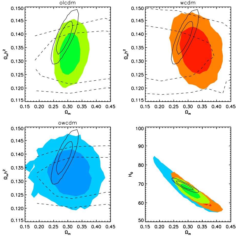
Figure 9. WMAP5+LRG constraints on \Omega_m h^2 , \Omega_m , and H_0 for \Lambda CDM (solid black contours), \text{o}\Lambda CDM (shaded green contours), \text{w}\Lambda CDM (shaded red contours), and \text{ow}\Lambda CDM (shaded blue contours) models. The first three panels show WMAP5-only constraints (dashed contours) and WMAP5+LRG constraints (colored contours) in the \Omega_m h^2 - \Omega_m plane as the model is varied. In the lower right we show all constraints from WMAP5+LRG for all four models in the \Omega_m - h plane, which lie within the tight \Omega_m h^2 \approx 0.133 WMAP5-only constraints.
