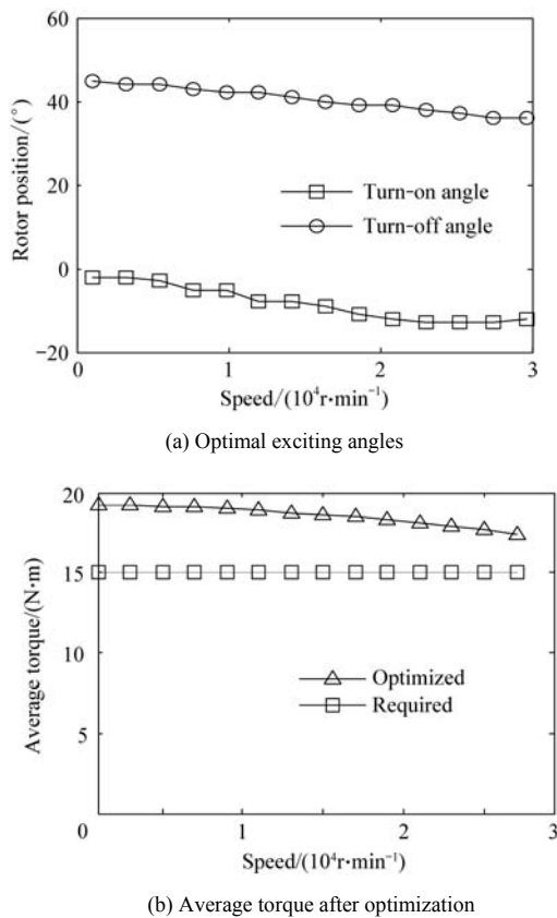
Fig.14 Optimization results in motoring mode.
