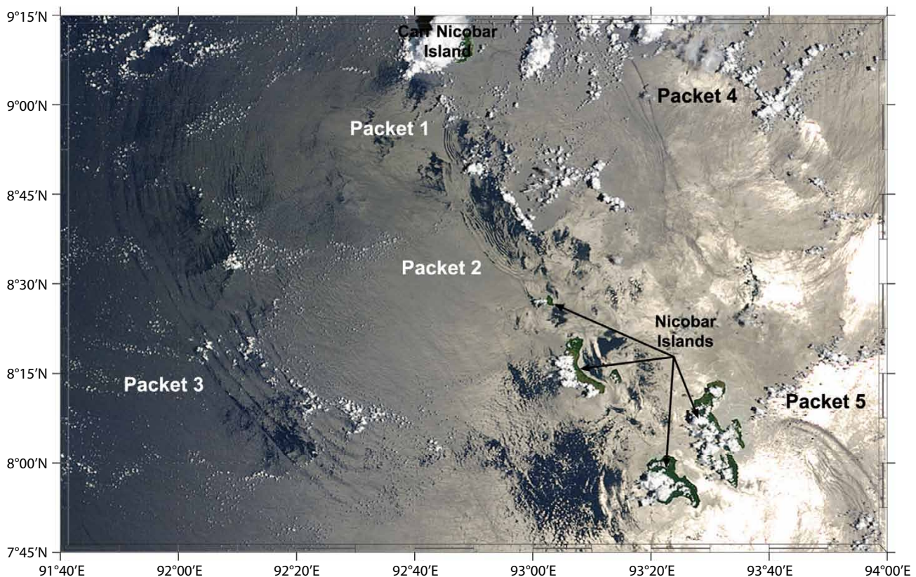
Figure 3. True-color MODIS image acquired on April 6, 2004, at 4:25 UTC showing the bidirectional generation of nonlinear internal waves from the sills among the Nicobar Island chain. Adapted from Jackson (2007)
