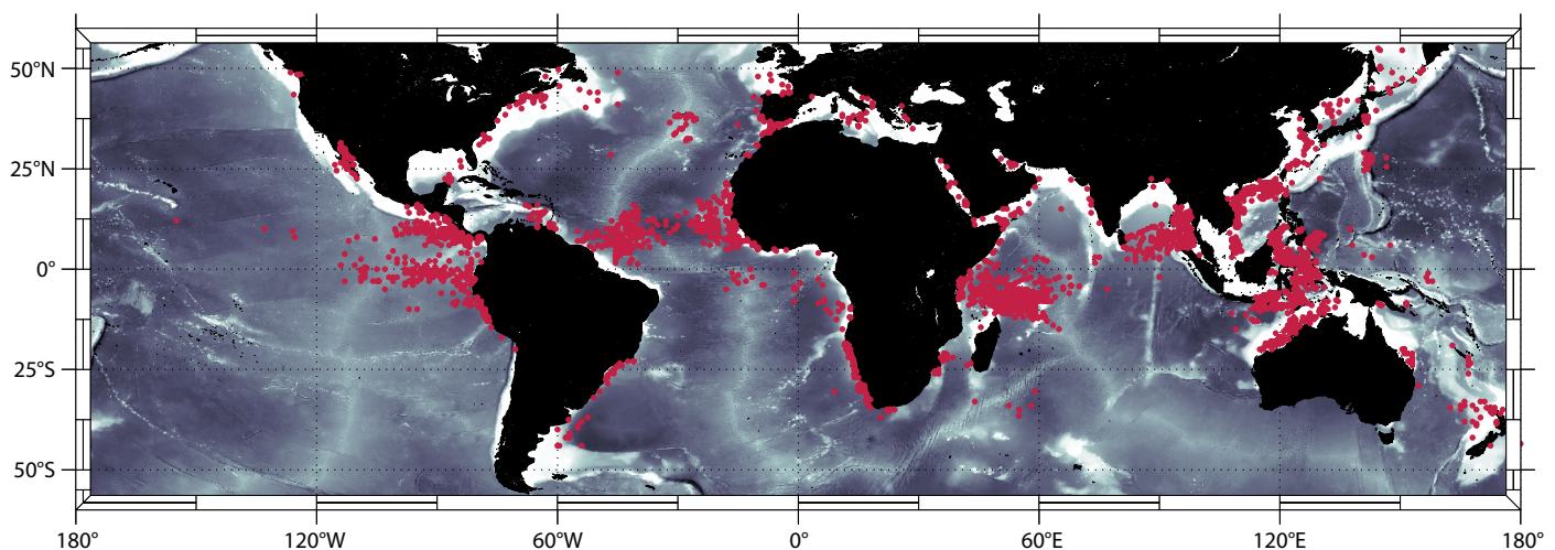
Figure 1. The location of nonlinear internal waves observed in 250 m resolution MODIS (Moderate-Resolution Imaging Spectroradiometer) satellite sunglint imagery acquired from August 2002 through May 2004. More than 3,500 nonlinear internal wave occurrences were identified by the survey. Adapted from Jackson (2007)
