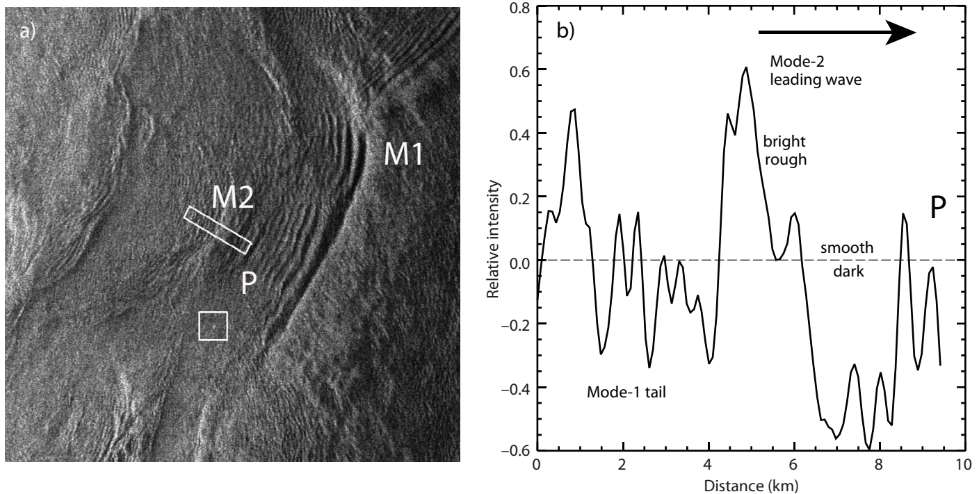
Figure 8. (a) Envisat ASAR image dated March 28, 2009, at 18:17 UTC of the Mascarene Plateau in the Indian Ocean. Labels M1 and M2 indicate signatures of mode-1 and mode-2 nonlinear internal waves. Profile P is shown in (b), where a mode-2 wave is followed by a tail of shorter-scale mode-1 internal waves (the white square represents an area unperturbed by internal waves from which P is normalized). (b) Radar backscatter profile P normalized with respect to a background area unaffected by nonlinear internal waves. A leading mode-2 solitary wave is identified by a dark signature preceding a bright signature in the direction of propagation (indicated by an arrow). Short-scale nonlinear internal waves follow the mode-2 larger wave in the form of a wave tail.
