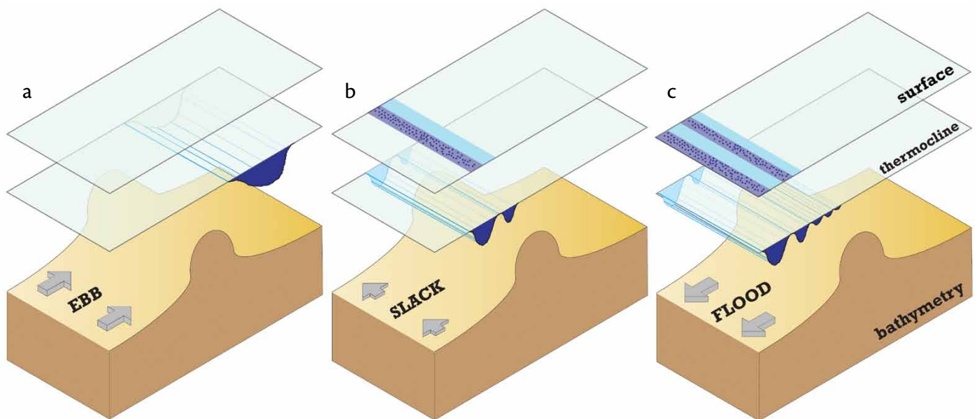
Figure 2. A schematic showing nonlinear internal wave generation via the lee wave mechanism of Maxworthy (1979). (a) As the stratified flow moves over the sill, the initial lee wave develops on the downstream side. (b) As the flow slackens, the lee wave steepens nonlinearly and propagates upstream over the sill. (c) The lee wave evolves into a nonlinear internal wave packet in a manner consistent with the predictions of Korteweg-de Vries theory. Adapted from Haury et al. (1979)
