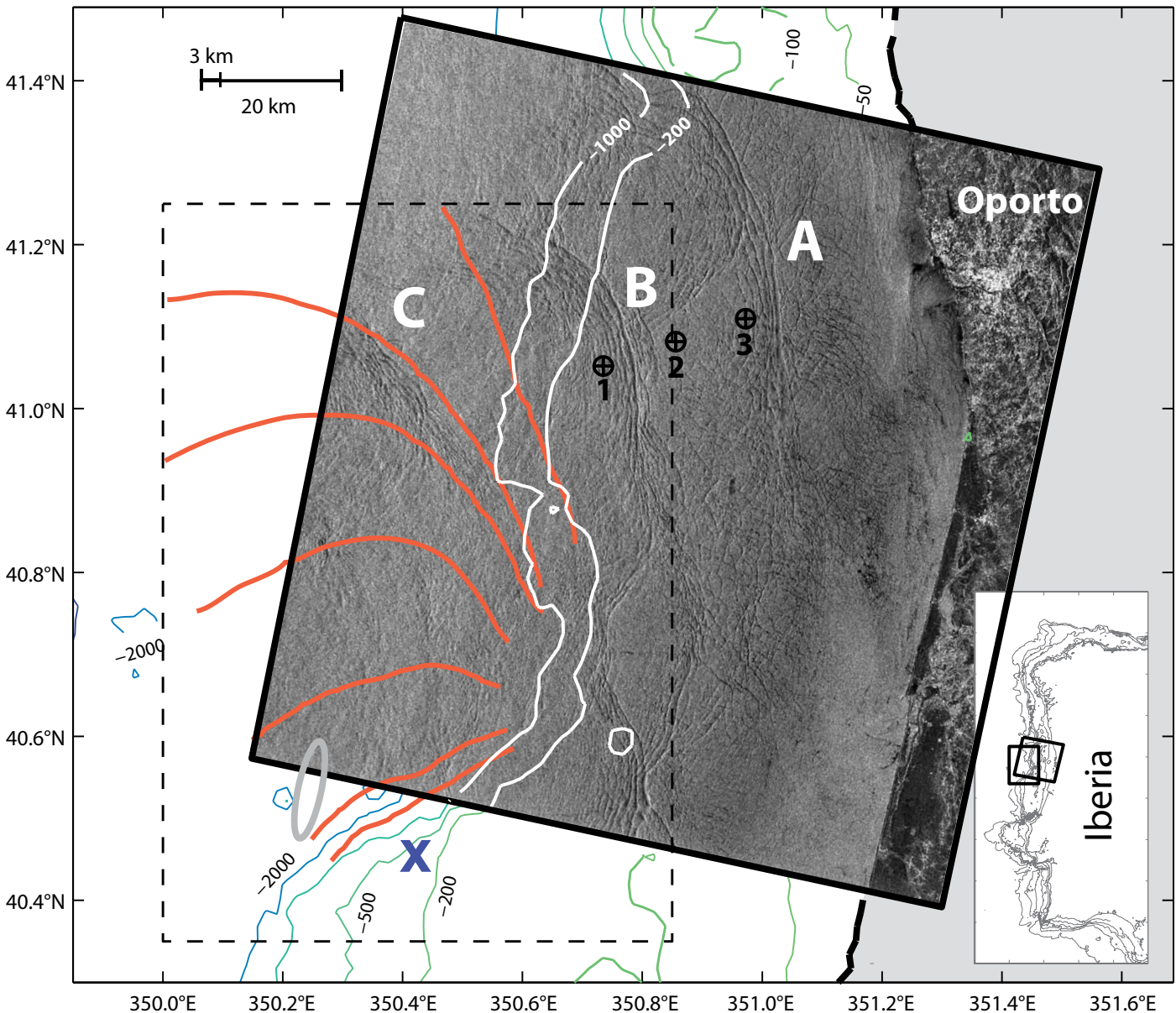
Figure 4. ERS-1 SAR (European Remote Sensing-1 synthetic aperture radar) image acquired August 8, 1994, at 11:20 UTC (orbit 16020, frame 2781). Light regions indicate high backscatter. The “X” denotes the generation site and the orange curves show the refraction of internal waves that propagate onshore to impact the shelf break. In situ measurements of nonlinear internal waves were made at the stations marked 1 to 3. The distance between the leading waves in the packets is approximately 500 m.
