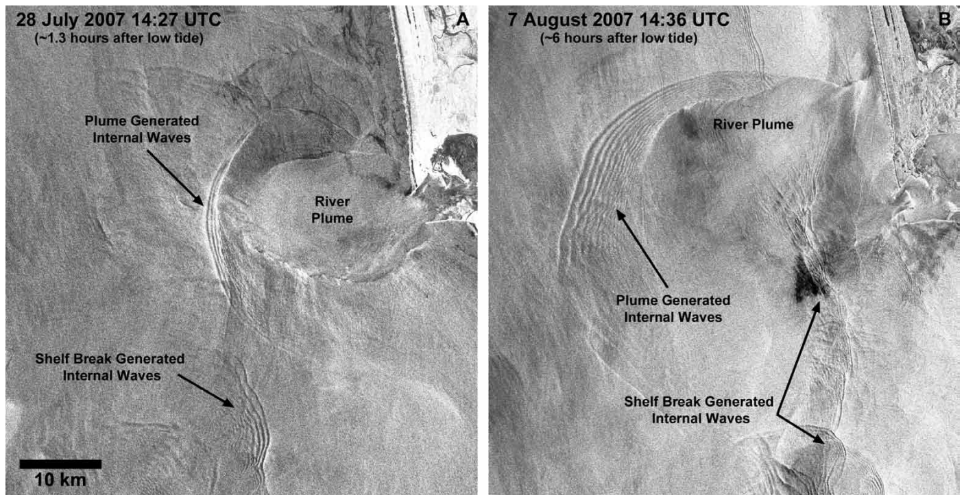
Figure 7. Radarsat-1 SAR images from July 28 and August 7, 2007, showing the evolution of nonlinear internal wave packet generated by the Columbia River plume.
