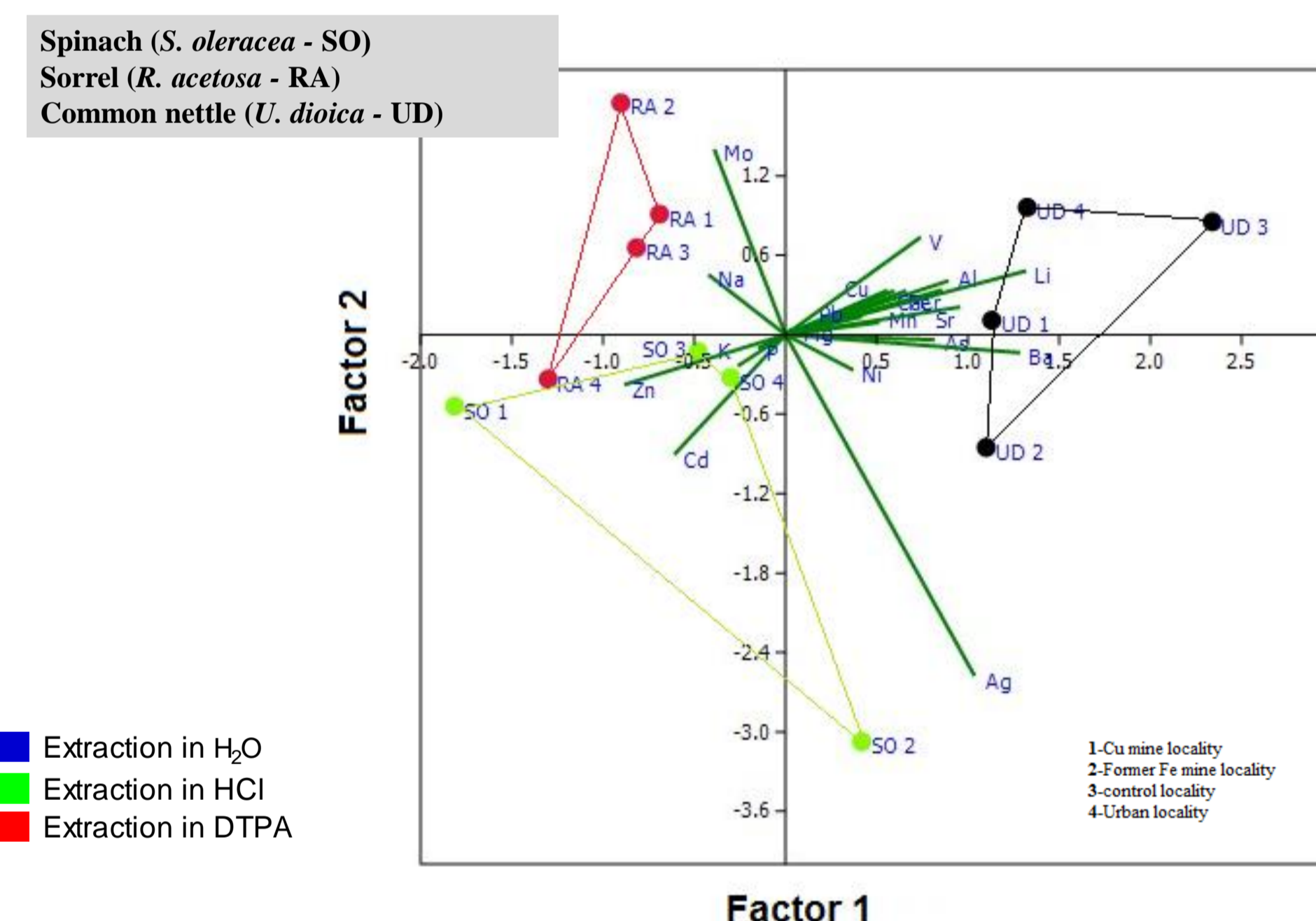
Figure 1. Principle components for type's vegetable and herb species and its elements contents; Site 1 and 2 – polluted area; Site 4 – urban area; Site 3 – control area
