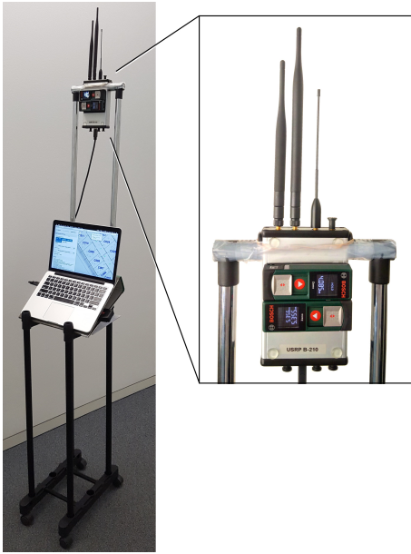
Fig. 2. Data acquisition cart with a USRP B210 receiver and ground-truth rangefinders [24].
