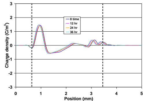
(b) Charge decay after negative voltage stressing
