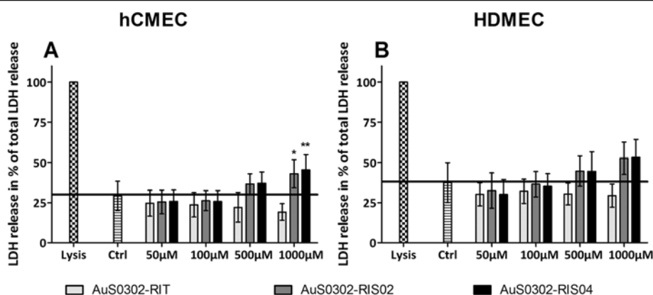
Figure 2 LDH release in hCMEC/D3 and HDMEC after 48 h exposure to AuNPs. The endothelial cells hCMEC/D3 (A) and HDMEC (B) were exposed to different amounts of gold nanoparticles (50 μM – 1000 μM) for 48 hours. Gold-induced cytotoxicity was measured by the LDH release into the supernatant by an enzymatic assay system. As positive control lysed cells were used and set at 100% (lysis). The spontaneous LDH releases of untreated cells are indicated by the black horizontal line. Each result represents the mean ± standard deviation of three independent experiments, each of these was performed at least in triplicates (ONEway ANOVA with Dunnetts t-test: * P < 0.5; ** P < 0.05; *** P < 0.001).
