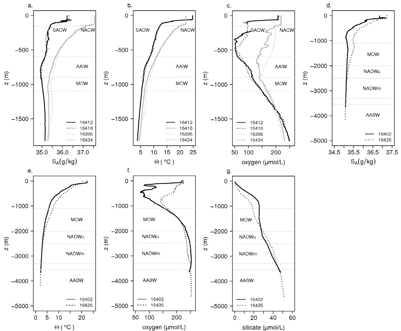
Figure 2. (a) Salinity ( S_A ), (b) conservative temperature ( \Theta ) and (c) oxygen profiles for st16412 and st16416 at \sim 12.5^{\circ}\text{N} , and st16395 and st16434 at \sim 25 – 27.5^{\circ}\text{N} and (d) salinity ( S_A ), (e) conservative temperature ( \Theta ), (f) oxygen and (g) silicate profiles for st16402 and st16435. Note that water mass designations are indicative only.
