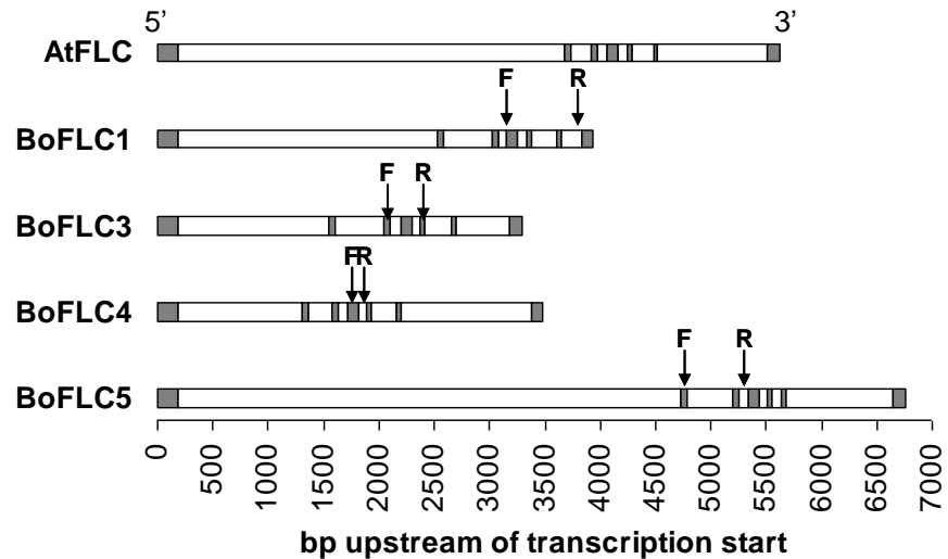
Figure 14: Diagrammatic representation of the structures of AtFLC , BoFLC1 , BoFLC3 , BoFLC4 , and BoFLC5 as described by Razi et al. (Razi et al. 2008). (The Genbank accession numbers for these genes are AF116528, AM231517, AM231518, AY306124, and AM231519 respectively). The exons are shaded in grey and the introns are white. The arrows indicate the exons in which the forward (F) and reverse (R) primers for each BoFLC homologue used in this study are located. The sizes of the introns and exons in each of these genes are given in Appendix 8. The cDNA sequences for BoFLC1 , BoFLC3 , BoFLC4 , and BoFLC5 are shown in Appendix 10.
