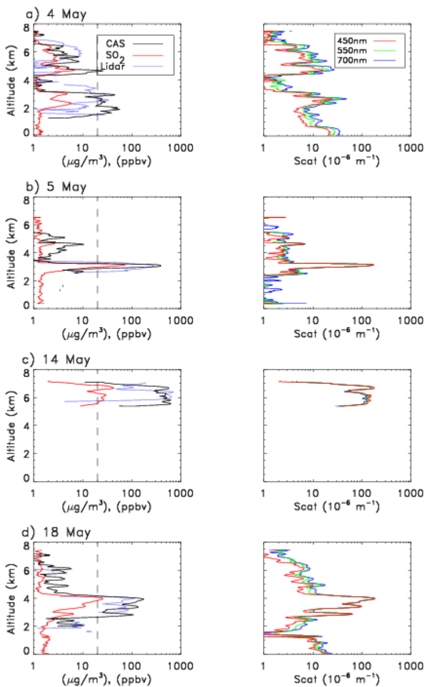
Figure 12. Vertical distributions of ash mass concentration derived from CAS and lidar (dashed line at the 20 \mu\text{g}/\text{m}^3 threshold used to define ash plume penetrations in this study), SO 2 concentration, and nephelometer scattering coefficients for selected aircraft profiles: (a) 4 May (B526), 51.5^\circ\text{N} 5.6^\circ\text{W} , 1240UTC, 1660km downwind; (b) 5 May (B527), 53.0^\circ\text{N} 5.1^\circ\text{W} , 1220UTC, 1530km downwind; (c) 14 May (B528), 59.6^\circ\text{N} 7.0^\circ\text{W} , 1240UTC, 840km downwind; (d) 18 May (B531), 56.5^\circ\text{N} 3.7^\circ\text{E} , 1145UTC, 1260km downwind.
