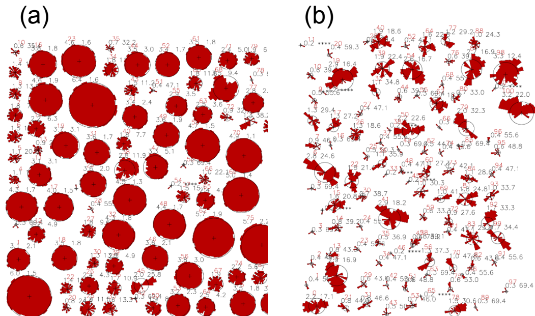
Figure 8. Azimuthal scattering patterns from the Small Ice Detector (SID-2H) probe on the FAAM aircraft for samples of aerosols found over the Irish sea at (a) 30m altitude and (b) 5km. The symmetric scattering patterns (a) indicate spherical aerosol (i.e. water droplets and/or hydrated sea salt) whereas the highly asymmetric patterns (b) indicate irregular non-spherical particles (i.e. ash). Pairs of black numbers above each pattern give particle radius (µm) and asphericity factor.
