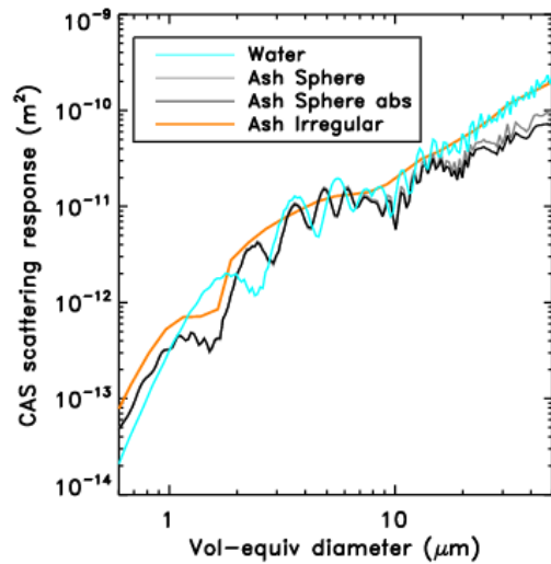
Figure 9. CAS scattering response (scattering cross-section, \text{m}^2 ) as a function of volume-equivalent diameter for water spheres ( \text{RI} = 1.33 + 0i ), ash spheres ( \text{RI} = 1.52 + 0.0015i ), more absorbing ash spheres ( \text{RI} = 1.59 + 0.004i ) and ash irregular-shaped particles ( \text{RI} = 1.52 + 0.0015i ).
