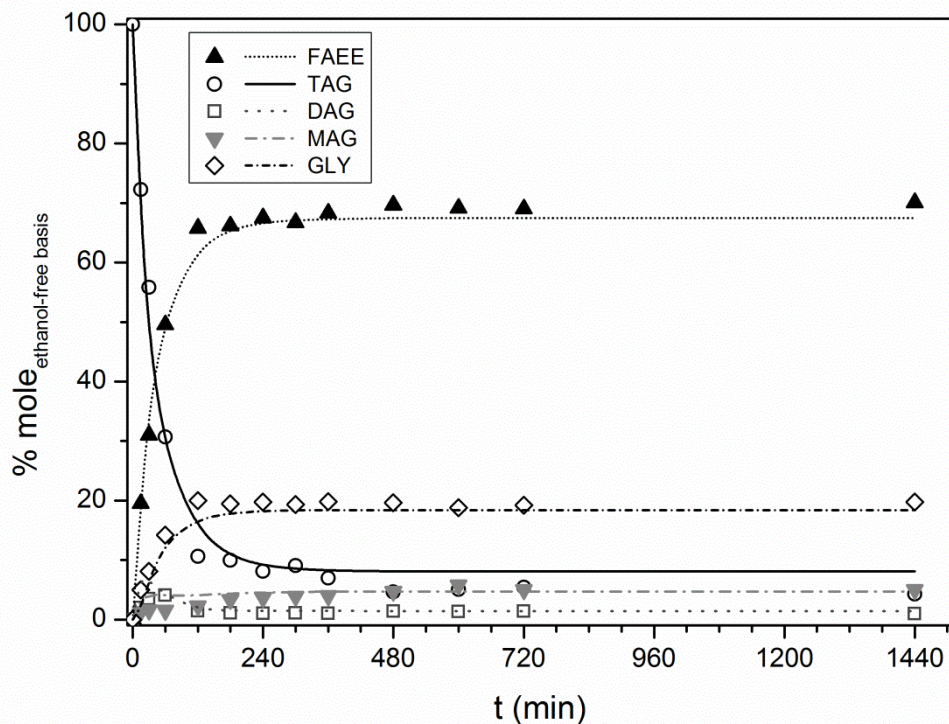
Figure 2. Components profile in the ethanolysis of fish oil catalyzed by Lipozyme RM IM in SC-CO 2 medium. Experimental conditions: MR = 38:1, p = 10 MPa, T = 323.15 K and enzyme loading 5 % wt. of substrates. FAEE: fatty acid ethyl esters, TAG: triacylglycerides, DAG: diacylglycerides, MAG: monoacylglycerides, GLY: glycerol. Lines represent the fitting of the proposed kinetic model to the experimental data.
