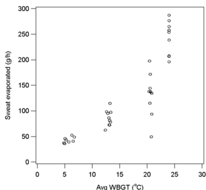
Figure 2. Sweat evaporated and the average WBGT in 60 minutes
