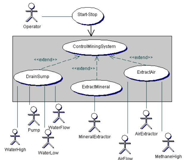
Figure 7 - Use case diagram for the MiningSystem
