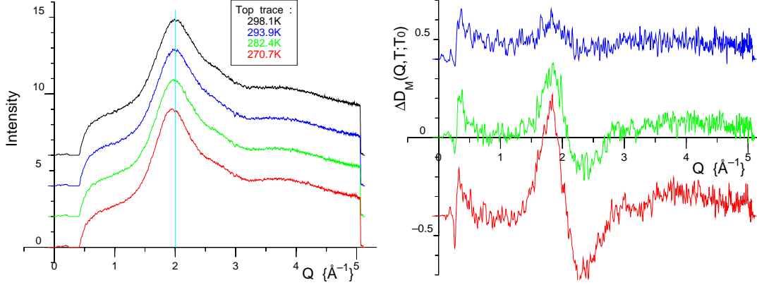
Figure 3. a) The diffraction pattern for the confined water at several temperatures (dry silica subtracted), b) the function, \Delta D_M(Q; \Delta T) , for the confined water with a reference temperature T_0=298\text{K} .
