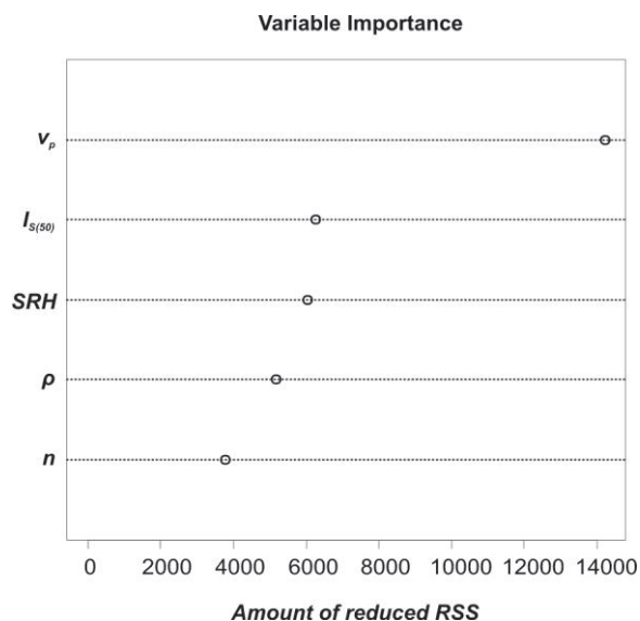
Figure 5: Importance of variables in a random forest due to the amount of reduced RSS
