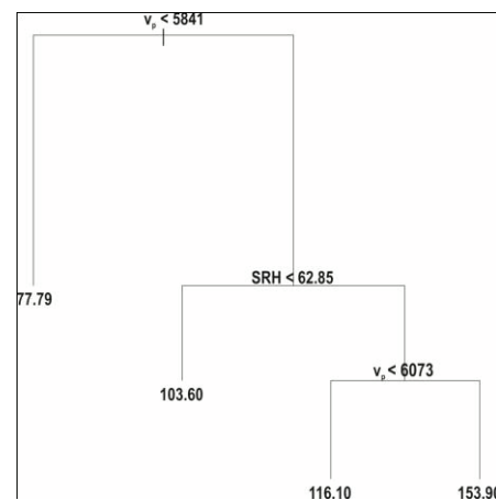
Figure 4: Regression tree model for estimation of the uniaxial compressive strength
