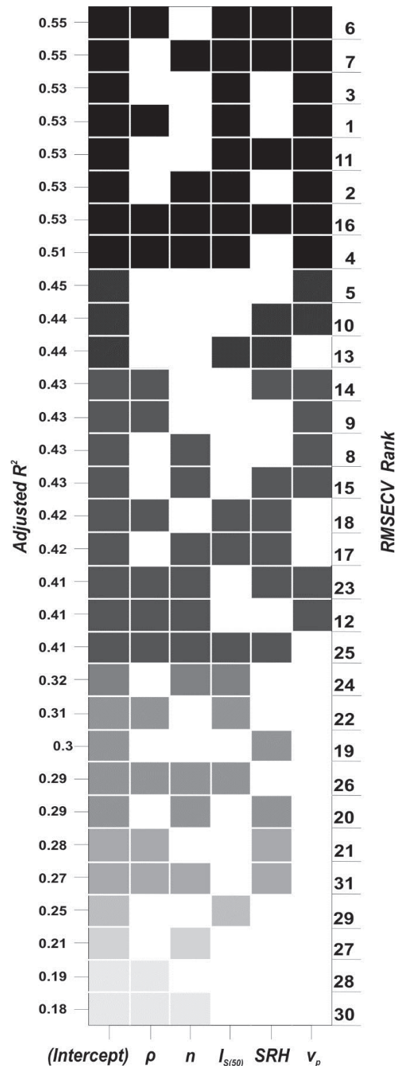
Figure 3 Rank of multiple linear regression models according to the adjusted R 2 and RMSECV
