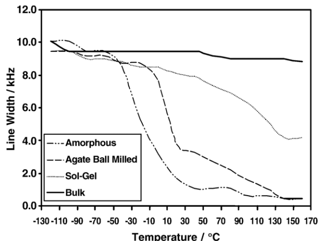
Fig. 7. The ^7\text{Li} NMR line width as a function of temperature for bulk, amorphous, sol-gel and ball milled \text{LiNbO}_3 .
