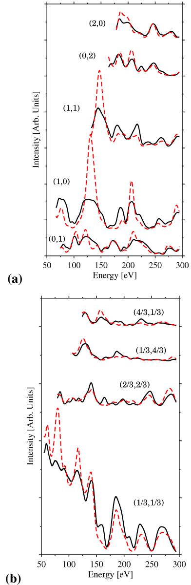
Fig. 5 Experimental (solid) and theoretical (dashed) LEED-IV curves for the best fit \text{Au}\{111\}-p(\sqrt{3} \times \sqrt{3})R 30^\circ\text{-I} structure: (a) integer (b) fractional order spots.
