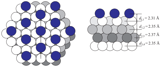
Fig. 3 Best-fit model of \text{Au}\{111\}-p(\sqrt{3} \times \sqrt{3})R 30^\circ\text{-Cl} . Left: top view, right: side view, cut along the [11\bar{2}] direction indicated by the dashed line in the top-view drawing. The Cl atoms are located in fcc adsorption sites (above the third layer gold atoms).
