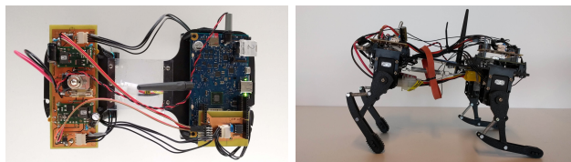
Fig. 1: Top down view and side view of Tigrillo.
