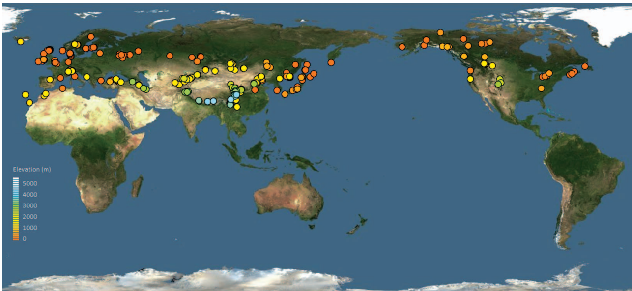
Fig. 1. Global distribution of sites for samples of the subgenus Bombus s. str. with accepted COI-barcode sequences (these bumblebees are not indigenous to subSaharan Africa, the Arabian peninsula, lowland India, southeast Asia, Australia or Central and South America). Spots are coloured to show the site elevation (scale in metres at left). Cartesian orthonormal projection, north at the top of the map.
