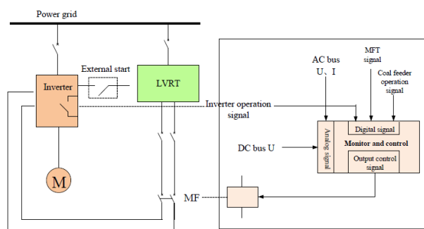
Fig. 22: Logic control of LVRT system [B3-0821(CN)]
