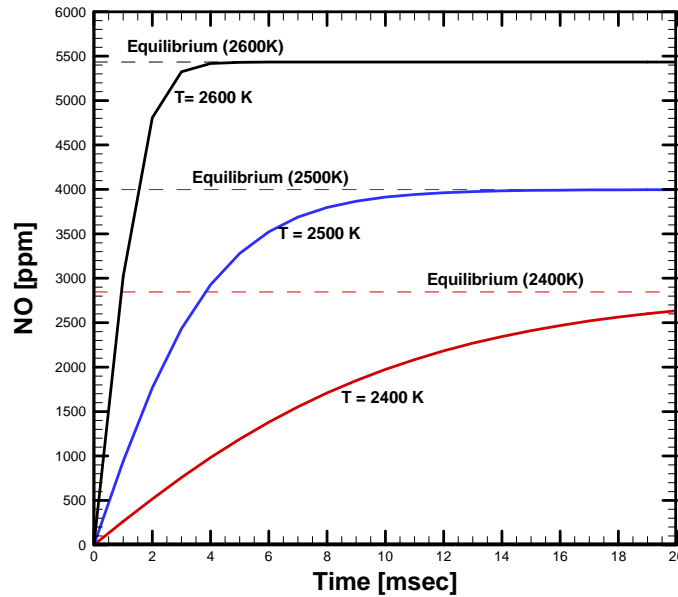
Figure 7 Nitric oxide concentration as a function of time and three equilibrium temperatures at 1000 kPa and an equivalence ratio of 1.0.
