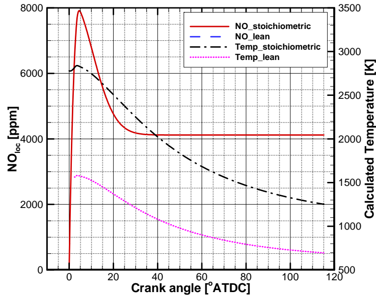
Figure 43 NO concentration for B20 at 1400 rev/min and 50 ft-lbs: (a) Zonal NO and temperatures, and (b) Averaged NO concentration.
