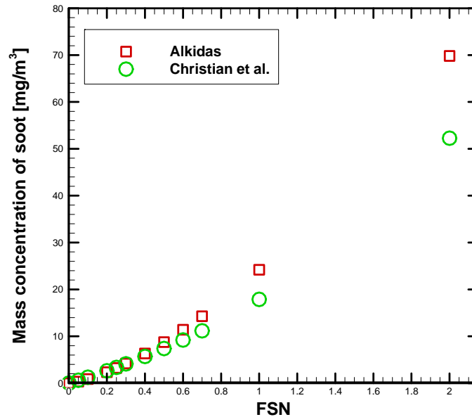
Figure 24 Mass concentration of soot calculated from FSN values.
