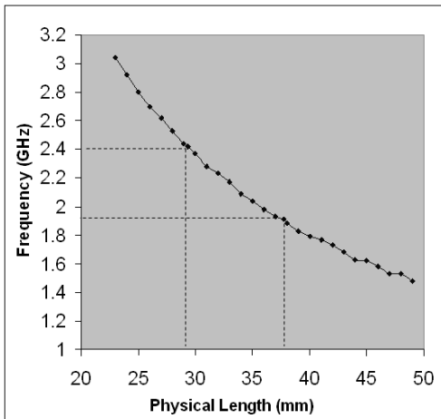
Fig.3 Physical length of the antenna in the frequency range 1-3 GHz
