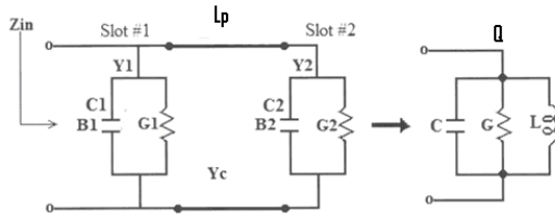
Fig.2 Transmission Line and Parallel Equivalent Circuits of the patch antenna
