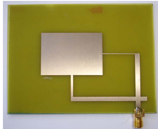
Fig.9 Photograph of the Fabricated Patch Antenna
