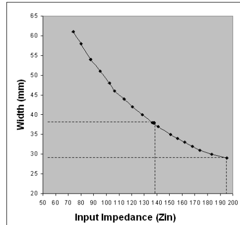
Fig.5 The edge input impedance at resonance as a function of the width of the patch.
