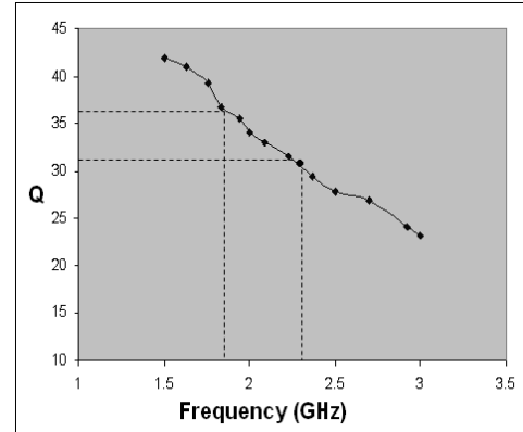
Fig.4 Q Factor of the antenna as a Function of Frequency
