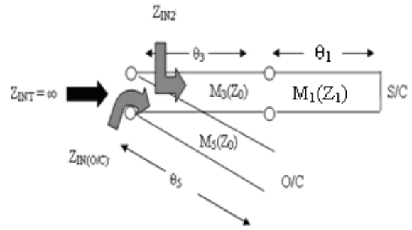
Figure.7 (b) Equivalent circuit to obtain matching at 2.4 GHz
