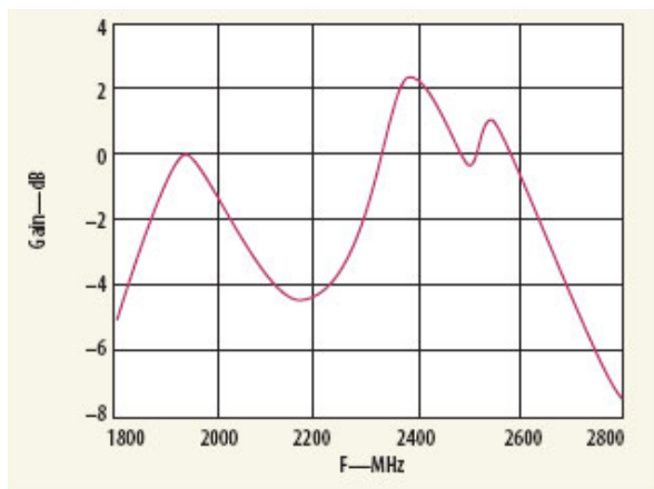
Fig.12 Frequency Response of the Gain of the Designed Antenna
