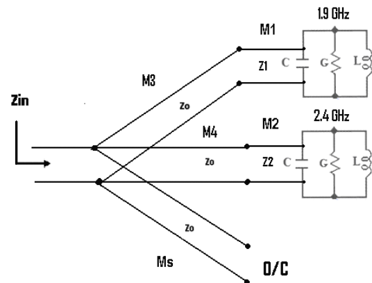
Fig.6 Equivalent Transmission Line Circuit of the Feed Network and Antenna
