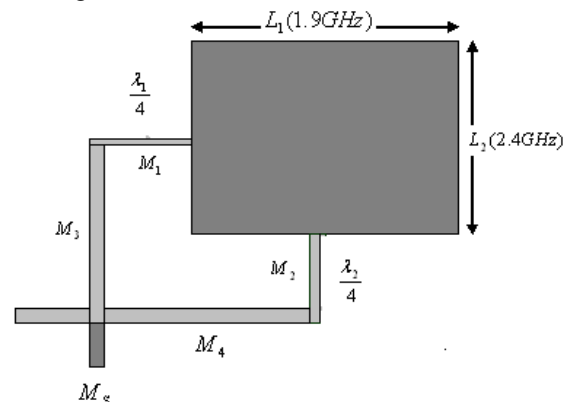
Fig.1 Antenna and the Feed Network
