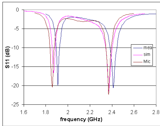
Fig.10 Practical and Simulated Results for the Return Loss
