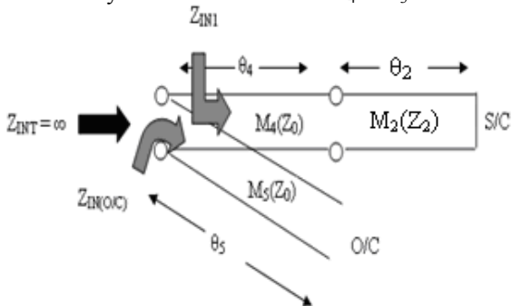
Figure.7 (a) Equivalent circuit to obtain matching at 1.9 GHz
