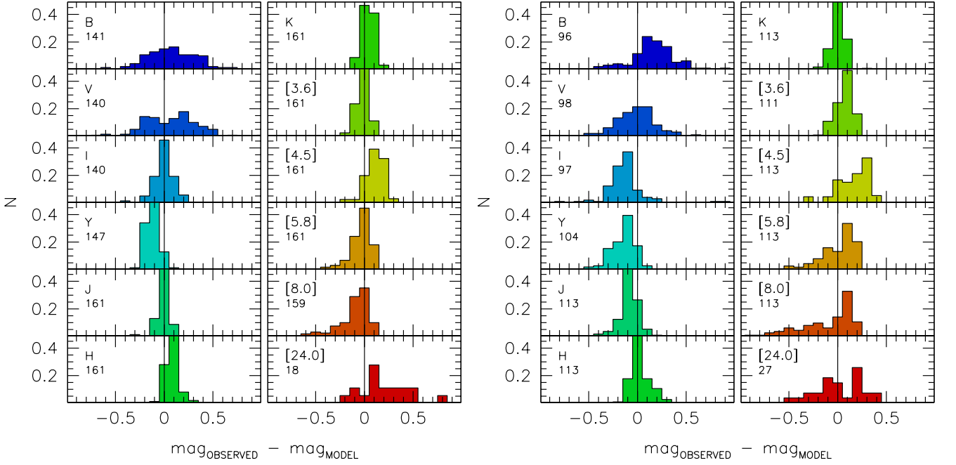
Fig. 3: Histograms of magnitude residuals for the data in all wave-bands, for O-rich ( left panel ) and C-rich ( right panel ) stars with J - K_s < 1.5 mag. The histograms are normalised to the total number of stars detected in each wave-band, labelled in each plot.
