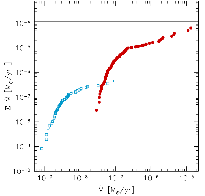
Fig. 8: Cumulative distribution of the mass-loss rates for O- ( open squares ) and C-rich ( filled dots ) AGB stars. The horizontal line shows the average mass-loss rates of the external regions of the LMC obtained by Matsuura et al. (2009), rescaled to the area encompassed by our analysis.
