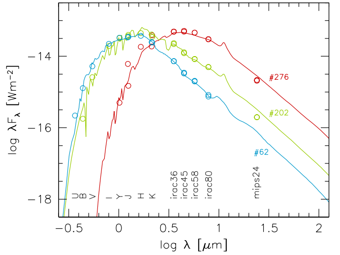
Fig. 2: Photometric data points ( open circles ) and the fitted SEDs ( lines ) for three AGB stars: a blue O-rich star ( J - K_s = 1.2 mag, id 62), and two C-rich stars ( J - K_s = 1.5 mag, id 202; and J - K_s \sim 4 mag, id 276).
