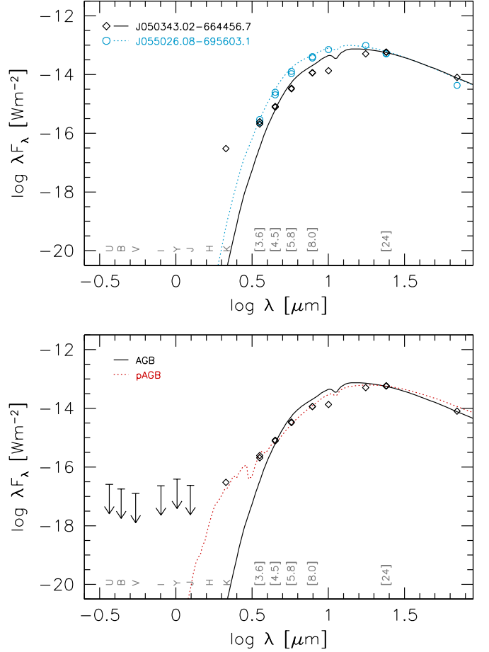
Fig. A.2: Photometric data points and standard AGB SED model for the Extremely Red Objects J050343.02-664456.7 ( diamonds and solid line ). In the upper panel they are compared with data and SED standard model for J055026.08-695603.1 ( circles and dotted line ). The lower panel show the post-AGB model with a detached dusty shell ( dotted line ). The arrows show the photometric detection limits.
