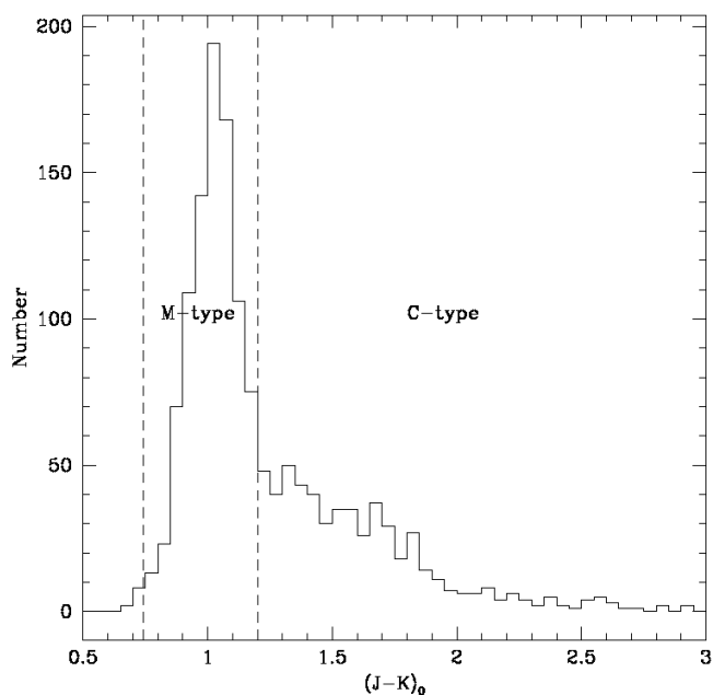
Fig. 10. Colour histogram with a bin size of 0.05 mag, of the AGB sources in the 17' \times 17' region used to determine the TRGB magnitude. The vertical dashed lines mark the positions of the blue limit at (J - K)_0 > 0.74 mag (Sect. 3.3.2) and the colour separation between the C- and M-type stars at (J - K)_0 = 1.20 mag.
