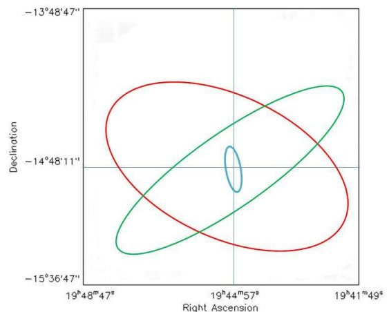
Fig. 1. Schematic diagram showing the relative scale and orientation of the three main structural components of NGC 6822. The bar of the galaxy (blue) (Hodge et al. 1991), the HI envelope (green) (de Blok & Walter 2000a; Battinelli et al. 2006) and the spheroid (red) (Battinelli et al. 2006)
