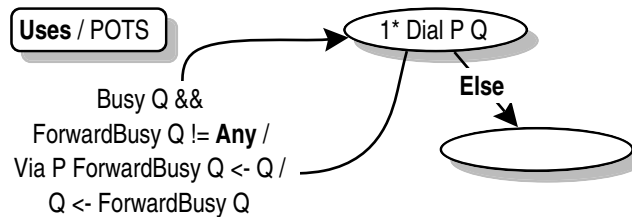
Figure 4: CRESS Feature Diagram for Call Forward on Busy Line
