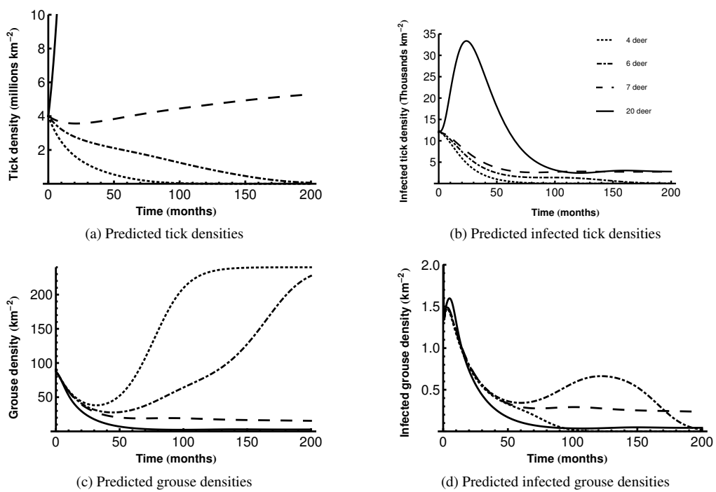
Figure 3: The effect of different deer densities on the effectiveness of sheep tick mops on a) tick, b) infected tick, c) grouse and d) infected grouse densities using the low sheep tick burden model. There are 50 sheep per \text{km}^2 treated with acaricide of 100% efficacy. The dotted line represents 4 deer per \text{km}^2 . The dot-dashed line represents 6 deer per \text{km}^2 . The dashed line represents 7 deer per \text{km}^2 . The solid line represents 20 deer per \text{km}^2 .
