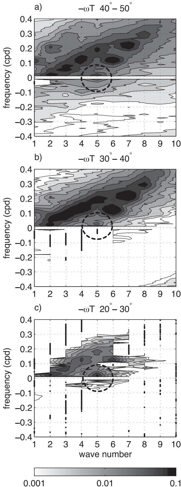
FIG. 8. As in Fig. 7b, but for the vertical heat transport at 500 hPa due to the meridionally averaged waves in the (a) 40^{\circ} – 50^{\circ} , (b) 30^{\circ} – 40^{\circ} , and (c) 20^{\circ} – 30^{\circ} latitude bands. The dotted circle points to the baroclinic energy conversion by the low-frequency wave 5. Note the inhibition in the central latitude band.
