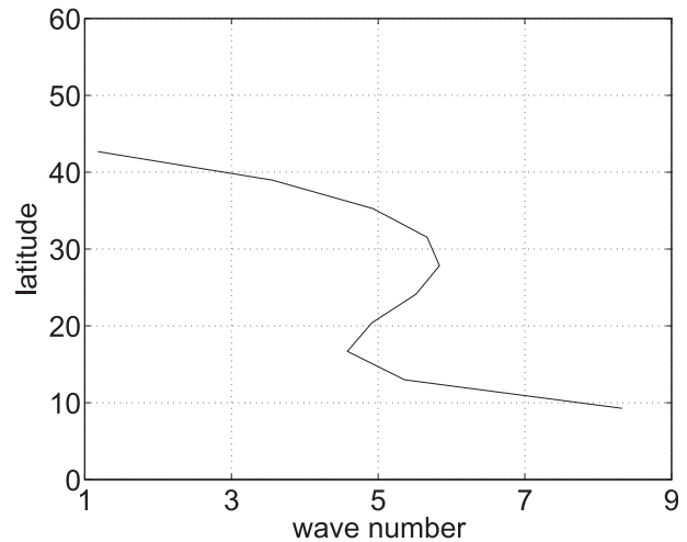
FIG. 11. Stationary Rossby wavenumber at 200 hPa as a function of the latitude. The increase observed around 30° is due to the meridional curvature of the zonal flow at the jet stream, which creates an upper tropospheric waveguide for a stationary Rossby wave 5.
