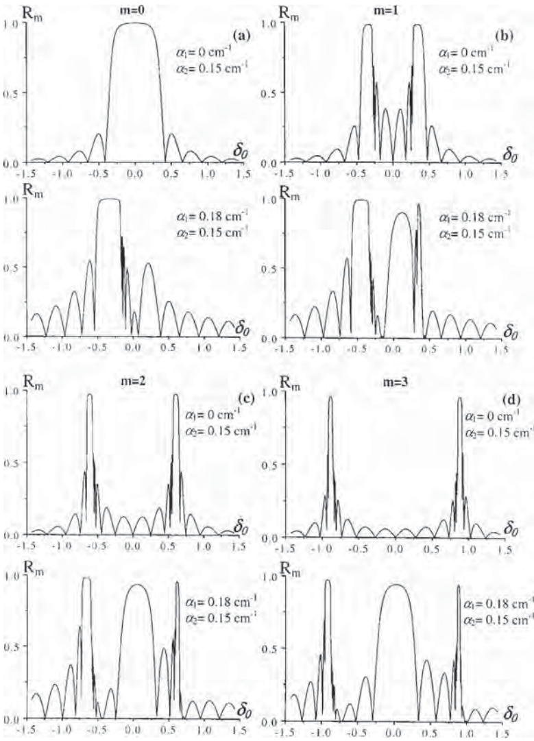
FIG. 6. The reflection coefficient from the ideal 2D SPBG structure (top figures) and 2D SPBG structure with a ‘‘rhombus’’ corrugation pattern (bottom figures) when l_z = 10 \text{ cm} , s = 0.29 \text{ cm}^{-1} , \sigma = 0.001 \text{ cm}^{-1} , and (a) m = 0 , (b) m = 1 , (c) m = 2 , and (d) m = 3 .
