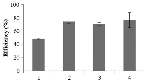
Fig. 9. Efficiency of precipitation; dc energization only. (1) Control (no HV). (2) +11 kV. (3) +14 kV. (4) +16 kV.
