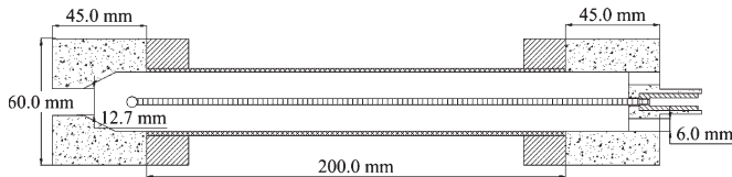
Fig. 1. Cross section of \mu -ESP reactor.
