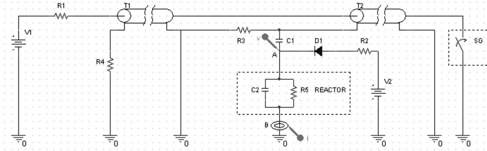
Fig. 2. Energization circuit used. SG stands for spark gap.
