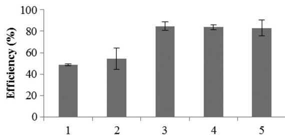
Fig. 10. Efficiency of precipitation; superposition of dc voltage and impulses. (1) Control (no HV). (2) +15.9-kV impulses only. (3) +11 kV dc with +26-kV impulses. (4) +14 kV dc with +29.3-kV impulses. (5) +16 kV dc with +30.9-kV impulses.
