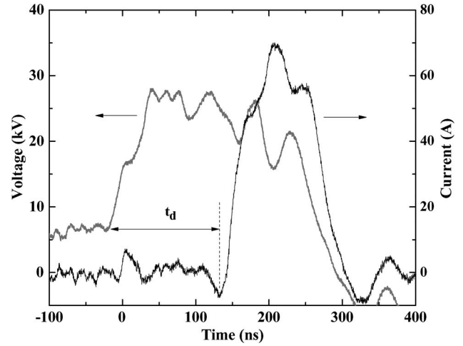
Fig. 4. Voltage impulse accompanied by a current impulse. t_d is the delay time between the HV impulse front and current impulse.
