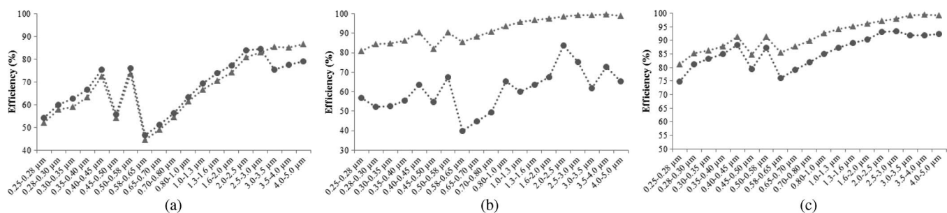
Fig. 11. Precipitation efficiency at (a) +11 kV dc and +24-kV-impulse energization, (b) +15 kV dc and +26-kV-impulse energization, and (c) +16 kV dc and +32-kV-impulse energization. (Circles) DC energization only. (Triangles) Superposition of dc voltage and HV impulses.
