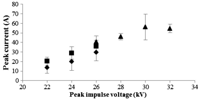
Fig. 6. Average peak impulse current as a function of applied impulse voltage for (diamonds) +11-kV-dc, (squares) +15-kV-dc, and (triangles) +16-kV-dc charging.
