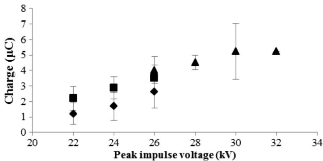
Fig. 7. Average charge injected as a function of impulse voltage for (diamonds) +11-kV-dc, (squares) +15-kV-dc, and (triangles) +16-kV-dc charging.
