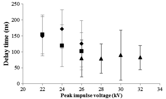
Fig. 5. Average time delay as a function of applied impulse voltage for (diamonds) +11-kV-dc, (squares) +15-kV-dc, and (triangles) +16-kV-dc charging.
