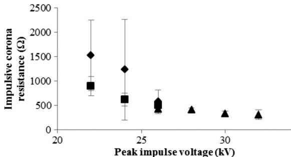
Fig. 8. Resistance at the peak of the current impulse as a function of impulse voltage for (diamonds) +11-kV-dc, (squares) +15-kV-dc, and (triangles) +16-kV-dc charging.
