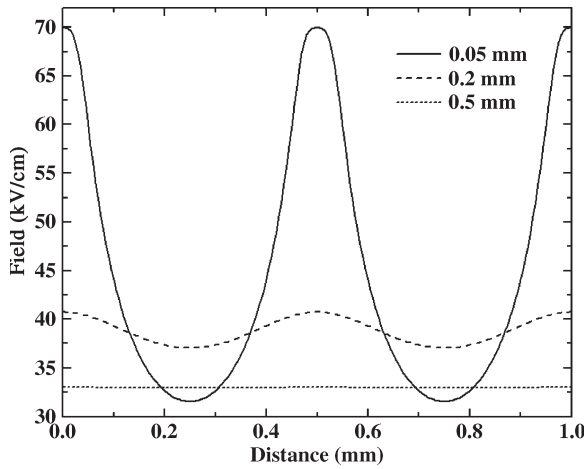
Fig. 3. Electric field along the threaded rod at distances of 0.05, 0.2, and 0.5 mm from the rod for +15-kV energization potential. The X -axis represents a section of the rod pitch M3.
