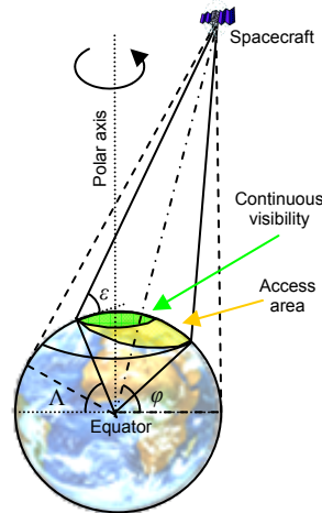
Fig. 3. Geometry of the spacecraft coverage. The yellow area is the surface covered with minimum elevation angle of \epsilon . The green area is the surface that is continuously visible from the spacecraft with the same minimum elevation angle: therefore \Lambda is the minimum latitude of continuous coverage.
