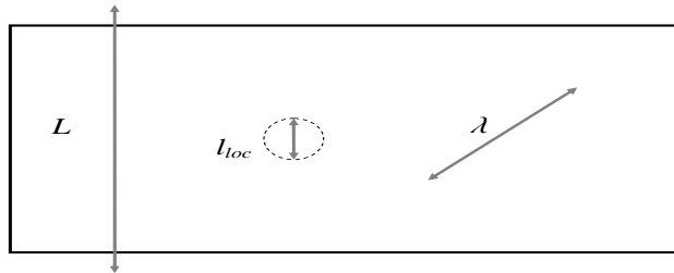
FIG. 1: Schematic of the three classical scaling parameters in gases
