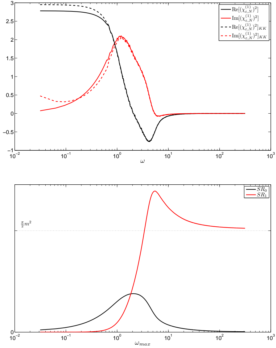
Figure 9: Properties of the square of the linear susceptibility \chi_{\epsilon, N}^{(1)} . The real and imaginary parts of [\chi_{\epsilon, N}^{(1)}]^2 with their KK transforms are depicted in the first panel, the vanishing sum rule for the real part and the non-vanishing sum rule for the imaginary part are depicted in the second panel.
